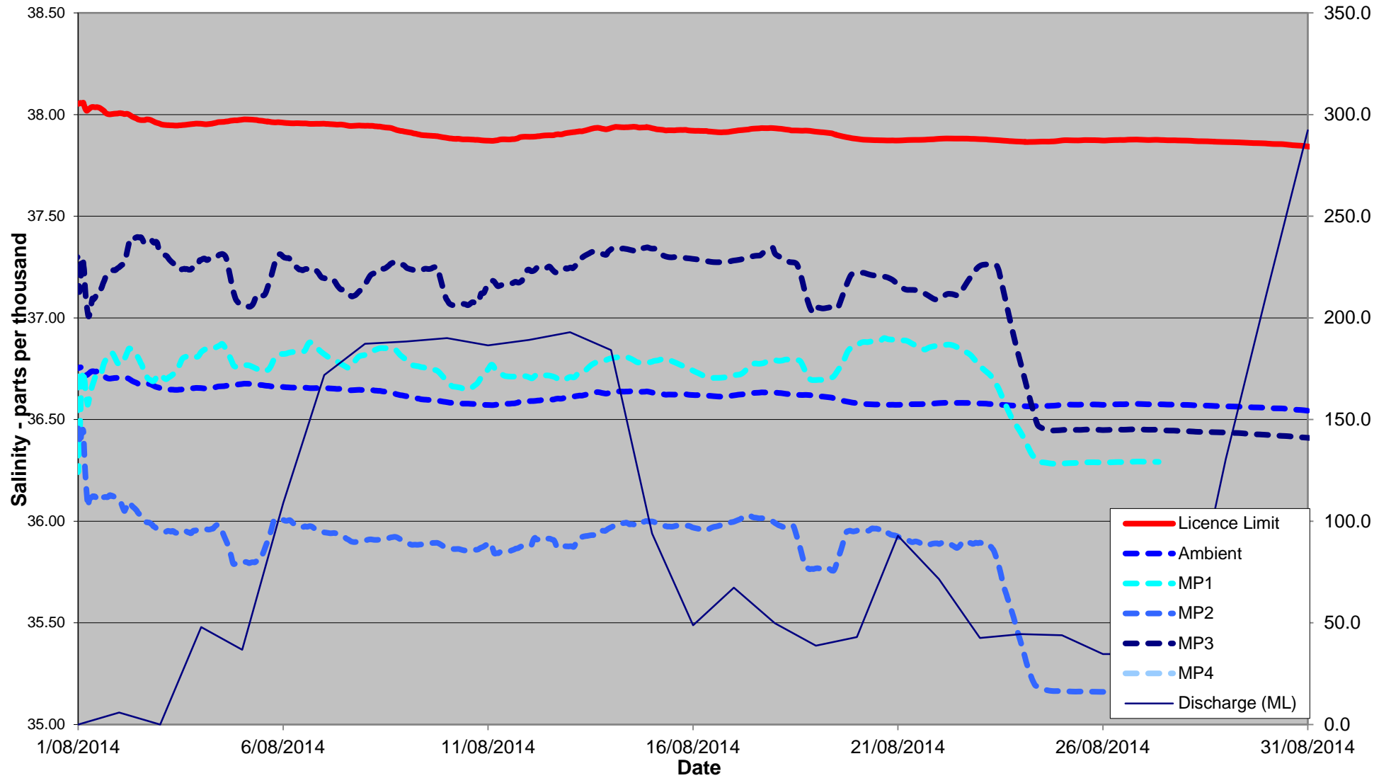
August 2014 24 Hour Average Salinity at 100 metres from Diffuser
