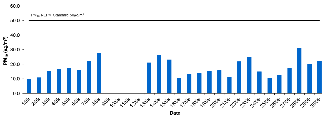
Le Fevre 1 Daily Average PM 10 - September 2014
