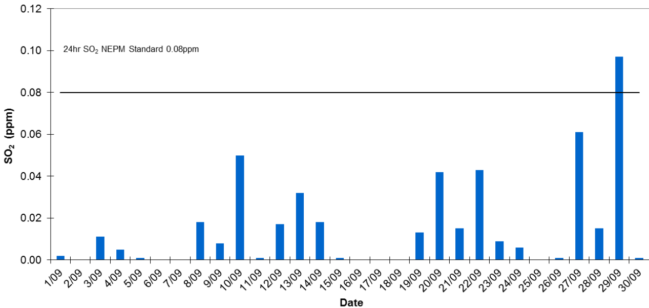
Pt Pirie Daily Average SO2 - September 2014
