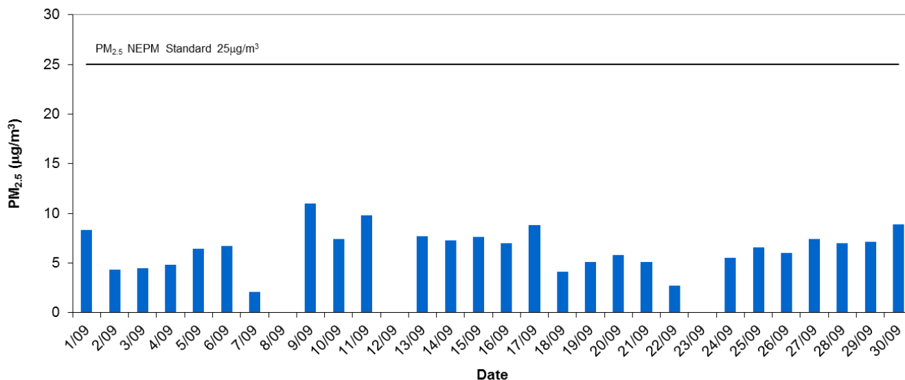
Adelaide CBD Daily Average PM2.5 - September 2014
