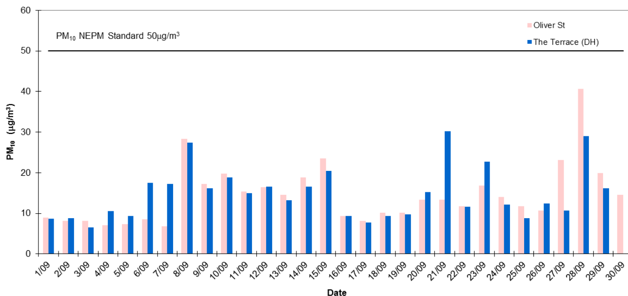
Pt Pirie Daily Average PM10 - September 2014
