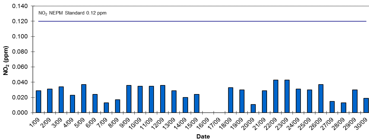
Adelaide CBD 1 Hr Daily Maxima NO2 - September 2014
