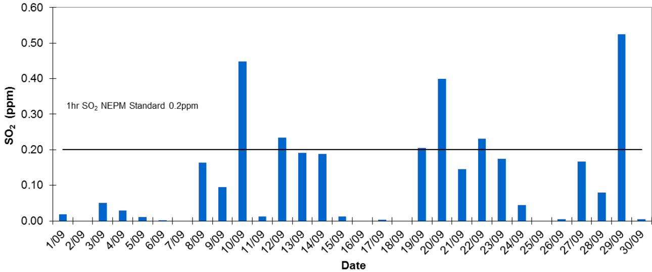
Pt Pirie 1 Hr Daily Maxima SO2 September 2014
