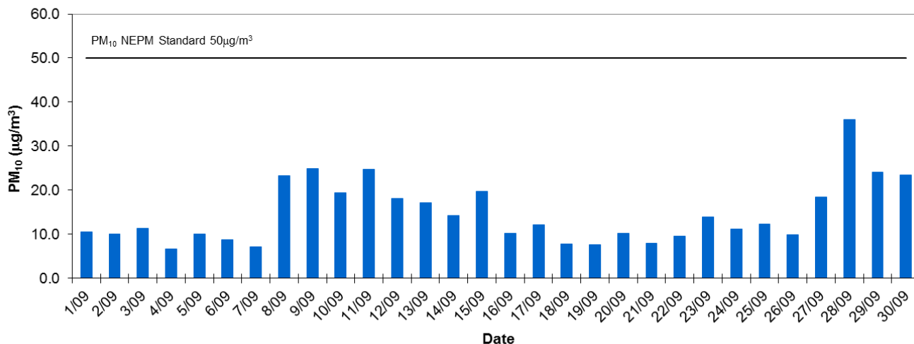
Southern Adelaide Daily Average PM10 - September 2014
