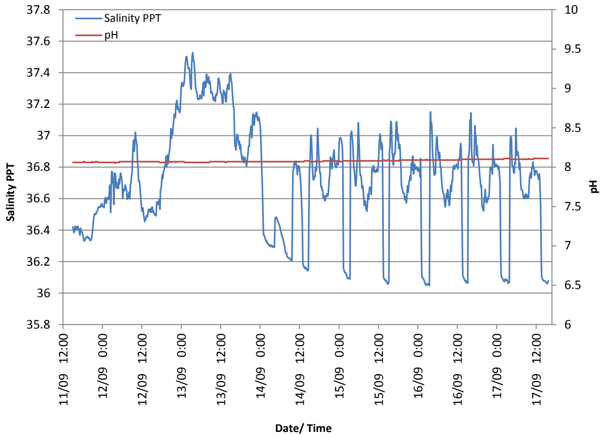
Figure 4. Changes in salinity (ppt) with pH over seven days, from 11 th September to 17 th September 2012.
