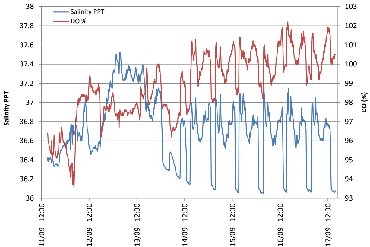
Figure 2. Changes in salinity (ppt) with dissolved oxygen (% saturation) over seven days, from 11 th September to 17 th September 2012.
