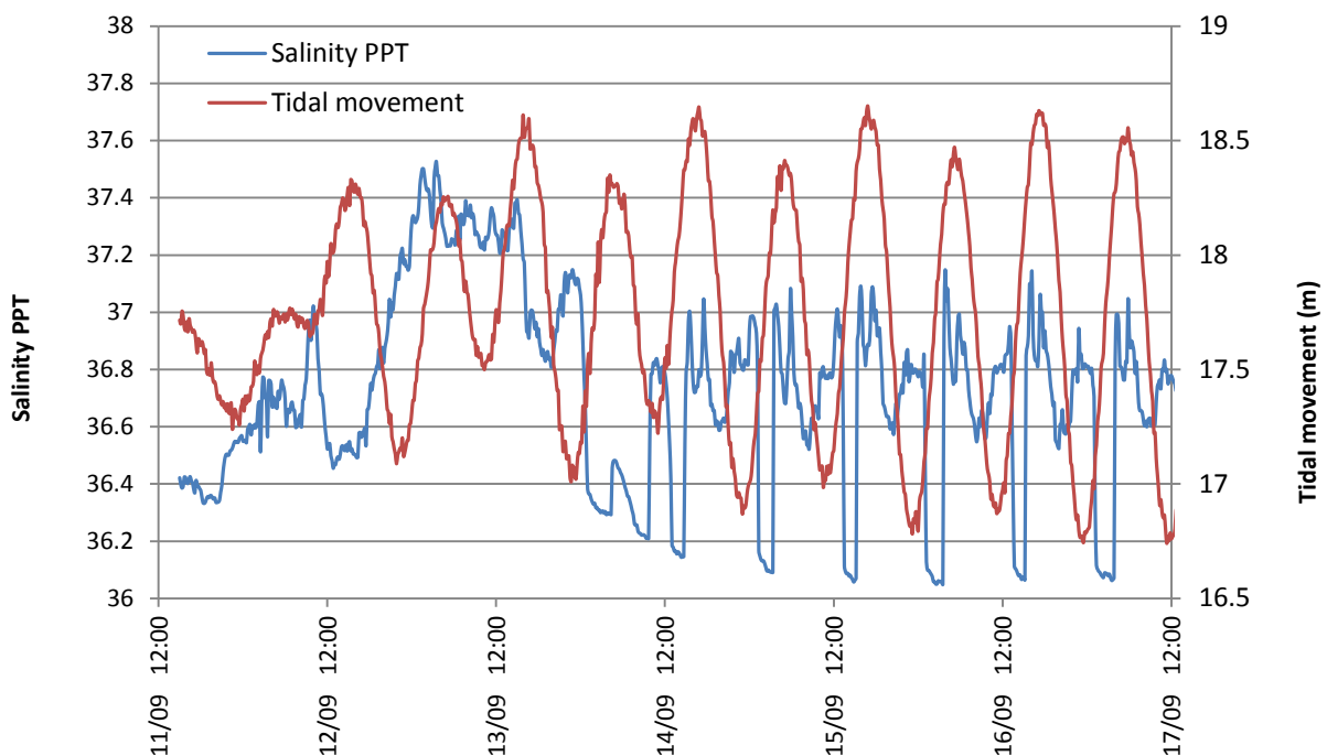
Figure 1. Changes in salinity (ppt) with tide (metres) over seven days, from 11 th September to 17 th September 2012.
