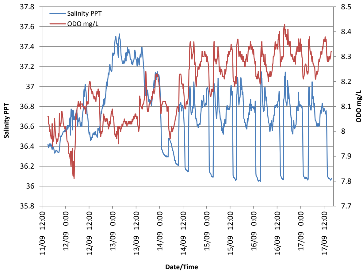
Figure 3. Changes in salinity (ppt) with dissolved oxygen (mg/L) over seven days, from 11 th September to 17 th September 2012.
