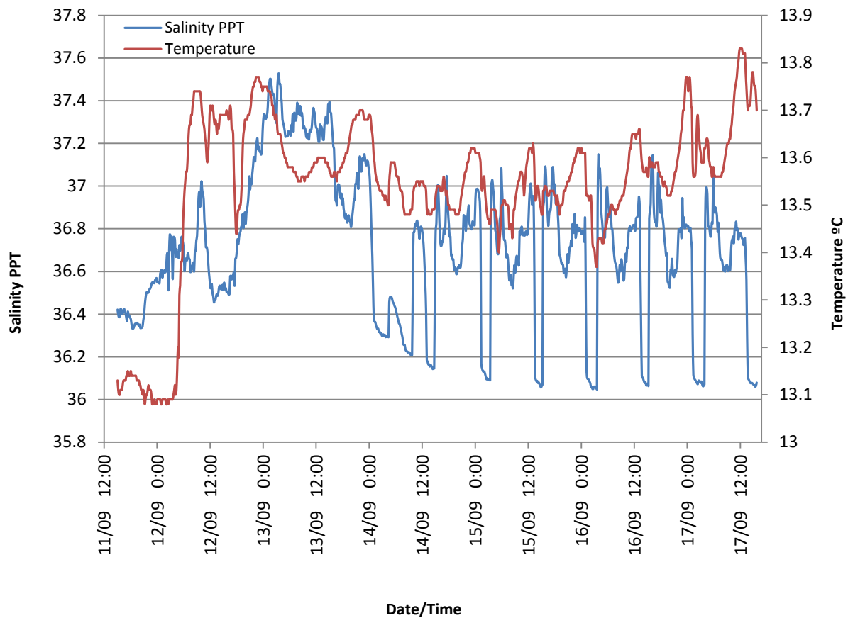
Figure 5. Changes in salinity (ppt) with temperature (°C) over seven days, from 11 th September to 17 th September 2012.
