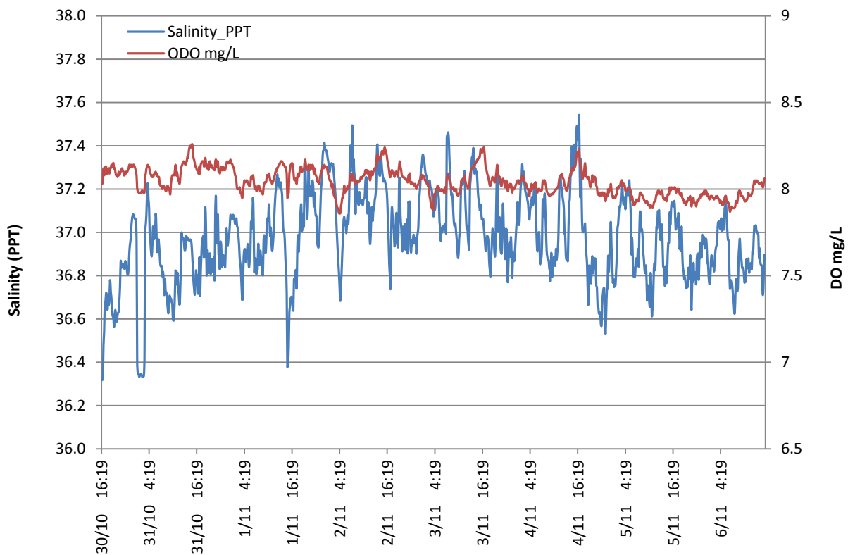
Figure 3. Changes in salinity (ppt) with dissolved oxygen (mg/L) over six days, from 30 th October to 6 th November 2012.
