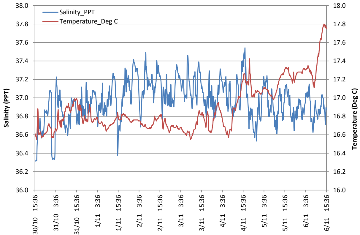
Figure 5. Changes in salinity (ppt) with temperature (°C) over six days, from 30 th October to 6 th November 2012.
