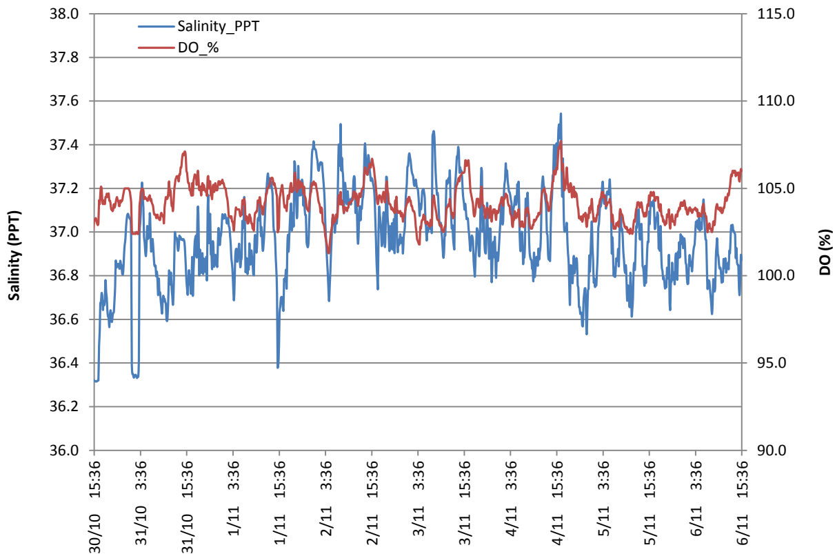
Figure 2. Changes in salinity (ppt) with dissolved oxygen (% saturation) over six days, from 30 th October to 6 th November 2012.
