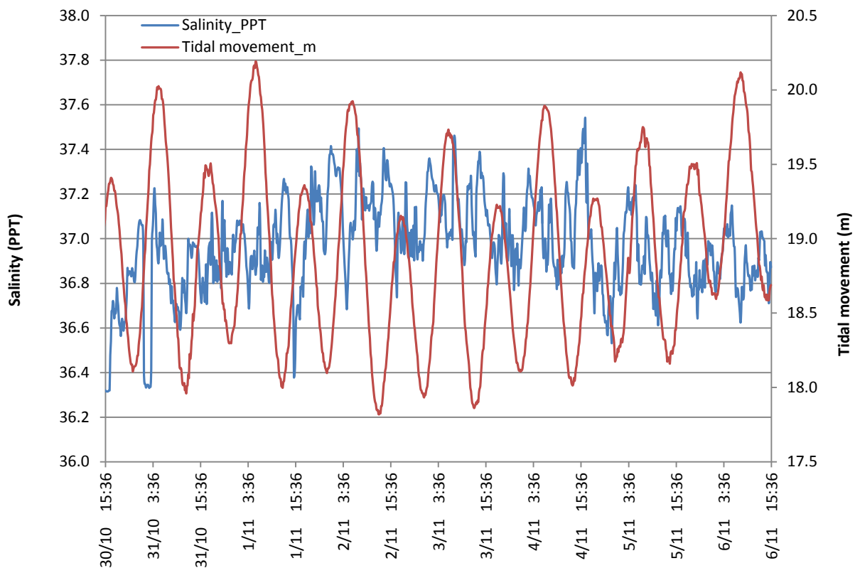
Figure 1. Changes in salinity (ppt) with tide (metres) over six days, from 30 th October to 6 th November 2012.
