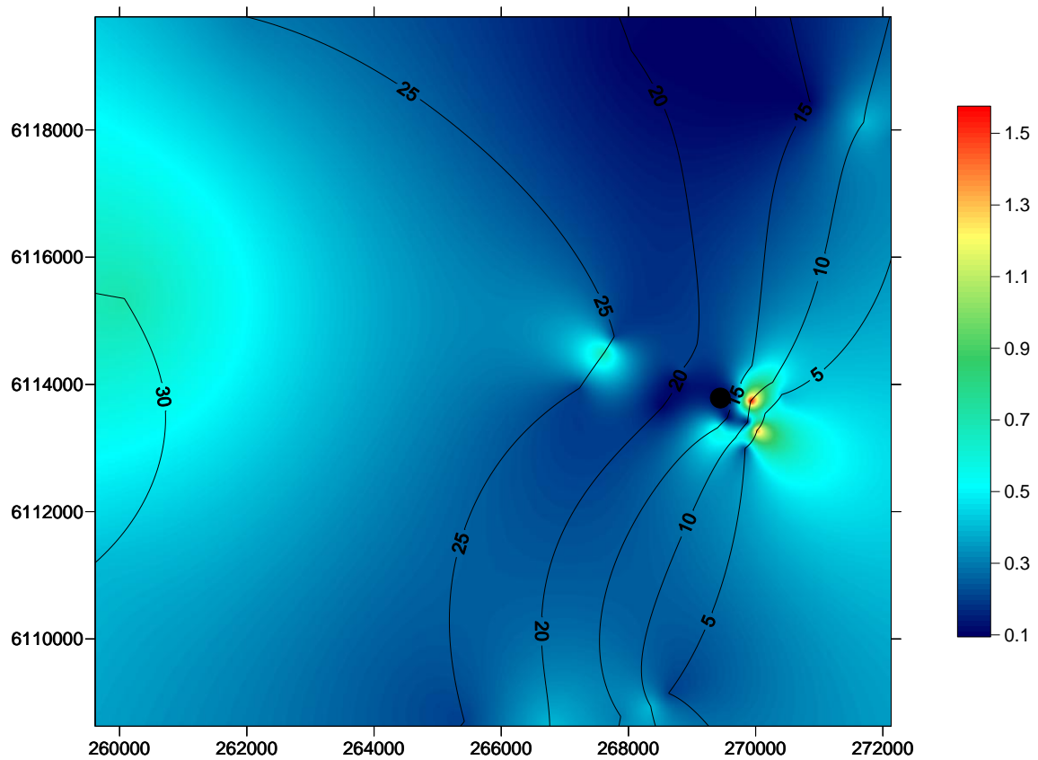
Figure 5 Spatial change in chlorophyll a concentration, one metre below the surface, in the Port Stanvac region. The coloured scale bar represents a change in chlorophyll concentration between 0.1 µg/L and 1.5 µg/L. Contour lines denote a five metre change in depth. X coordinates refer to eastings and Y coordinates refer to northings measured in metres. Black dot represents position of ADP outfall. Water quality survey undertaken on the 13th November, 2009.
