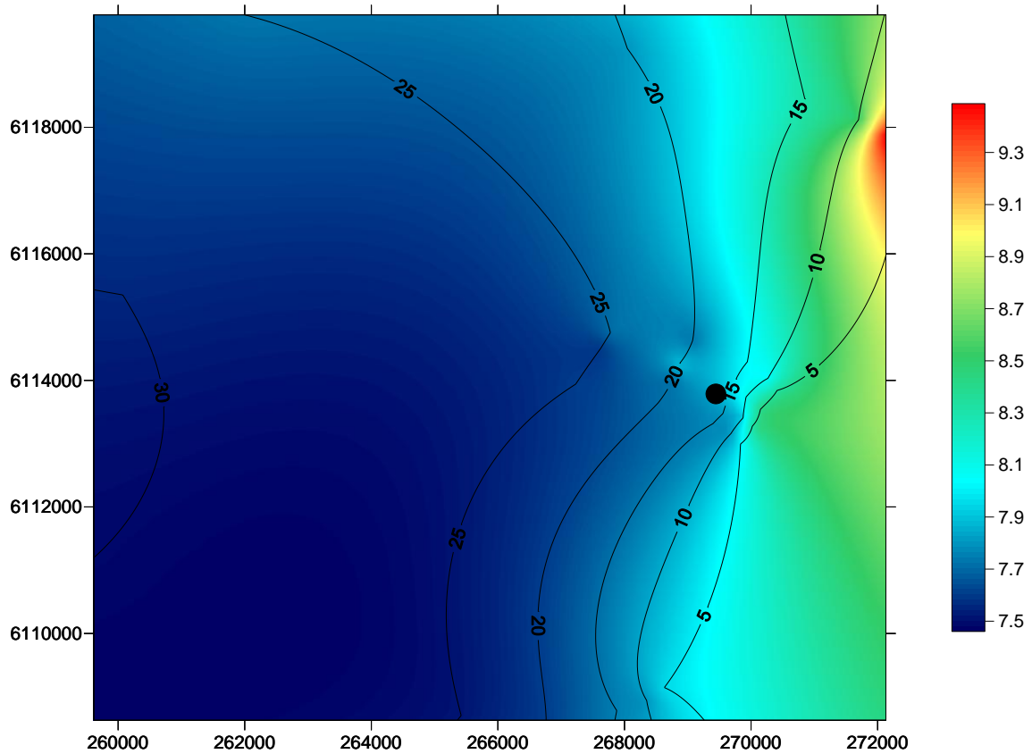
Figure 3 Spatial change in dissolved oxygen concentration, on the seafloor, in the Port Stanvac region. The coloured scale bar represents a change in the dissolved oxygen concentration between 7.5 mg/L and 9.3 mg/L. Contour lines denote a five metre change in depth. X coordinates refer to eastings and Y coordinates refer to northings measured in metres. Black dot represents position of ADP outfall. Water quality survey undertaken on the 13th November, 2009.
