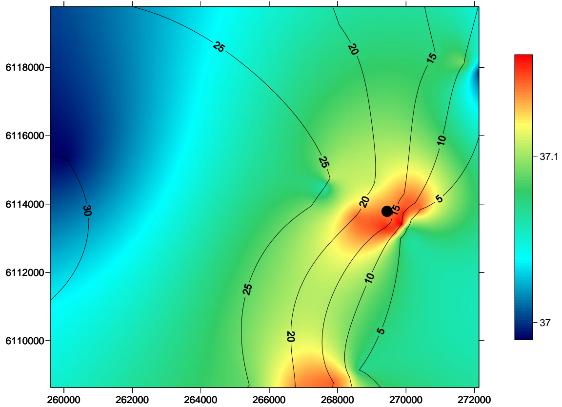
Figure 1 Spatial change in TDS (g/L) concentration, on the seafloor, in the Port Stanvac region. The coloured scale bar represents changes in TDS concentration between 37.0 g/L and 37.2 g/L. Contour lines denote a five metre change in depth. X coordinates refer to eastings and Y coordinates refer to northings measured in metres. Black dot represents position of ADP outfall. Water quality survey undertaken on the 13th November, 2009.
