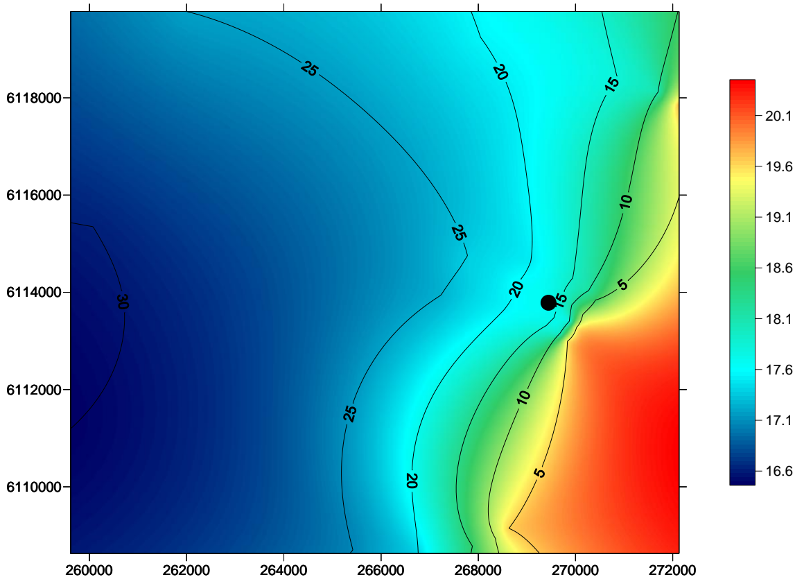
Figure 2 Spatial change in water temperature, on the seafloor, in the Port Stanvac region. The coloured scale bar represents temperature changes between 16.6 °C and 20.1 °C. Contour lines denote a five metre change in depth. X coordinates refer to eastings and Y coordinates refer to northings measured in metres. Black dot represents position of ADP outfall. Water quality survey undertaken on the 13th November, 2009.
