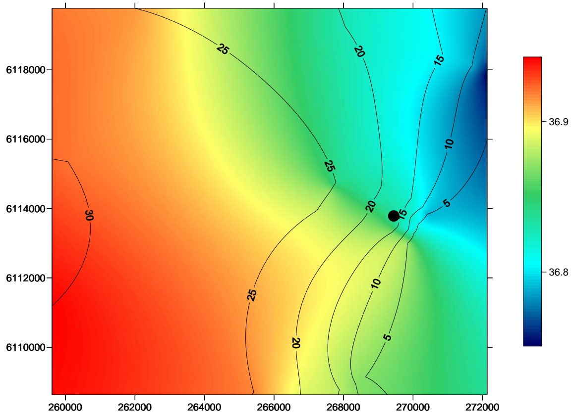
Figure 1 Spatial change in TDS (g/L) concentration, on the seafloor, in the Port Stanvac region. The coloured scale bar represents changes in TDS concentration between 36.7 g/L and 37.0 g/L. Contour lines denote a five metre change in depth. X coordinates refer to eastings and Y coordinates refer to northings measured in metres. Black dot represents position of ADP outfall. Water quality survey undertaken on the 27th October, 2010.
