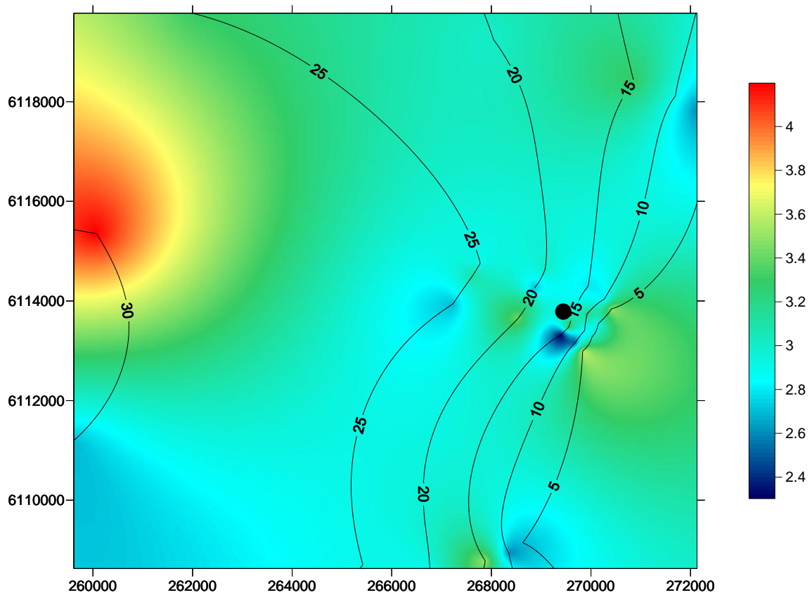
Figure 5 Spatial change in chlorophyll a concentration, one metre below the surface, in the Port Stanvac region. The coloured scale bar represents a change in chlorophyll concentration between 2.4 µg/L and 4.1 µg/L. Contour lines denote a five metre change in depth. X coordinates refer to eastings and Y coordinates refer to northings measured in metres. Black dot represents position of ADP outfall. Water quality survey undertaken on the 27th October, 2010.
