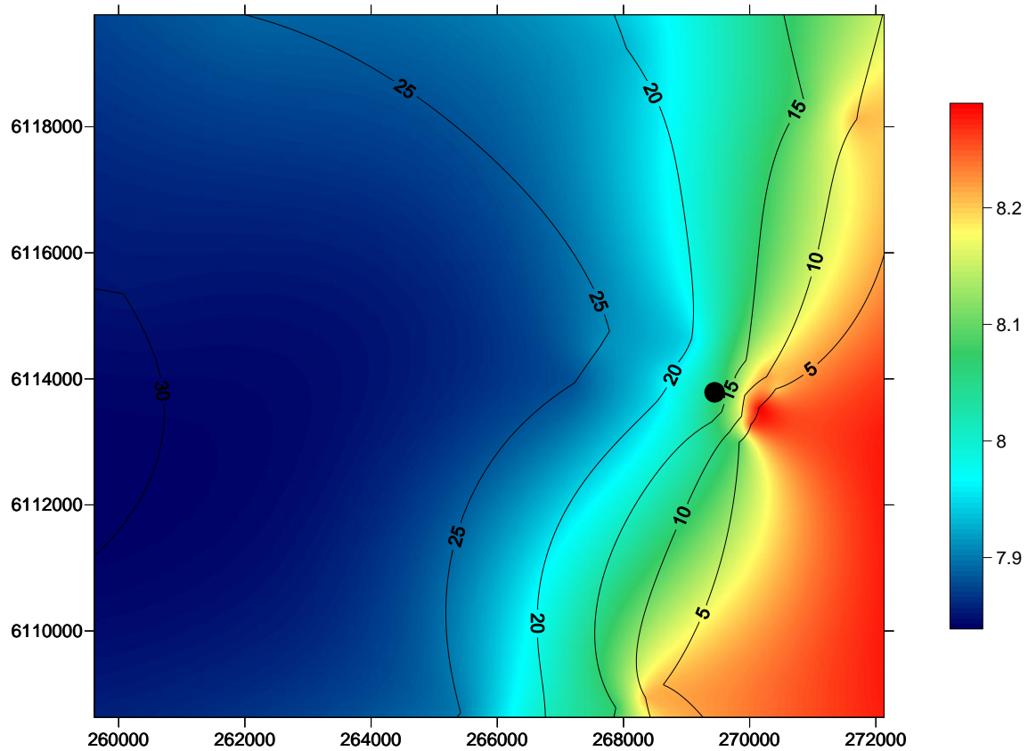
Figure 3 Spatial change in dissolved oxygen concentration, on the seafloor, in the Port Stanvac region. The coloured scale bar represents a change in the dissolved oxygen concentration between 7.8 mg/L and 8.3 mg/L. Contour lines denote a five metre change in depth. X coordinates refer to eastings and Y coordinates refer to northings measured in metres. Black dot represents position of ADP outfall. Water quality survey undertaken on the 27th October, 2010.
