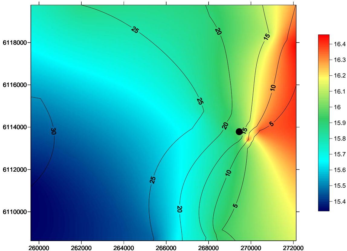
Figure 2 Spatial change in water temperature, on the seafloor, in the Port Stanvac region. The coloured scale bar represents temperature changes between 15.4 °C and 16.4 °C. Contour lines denote a five metre change in depth. X coordinates refer to eastings and Y coordinates refer to northings measured in metres. Black dot represents position of ADP outfall. Water quality survey undertaken on the 27th October, 2010.
