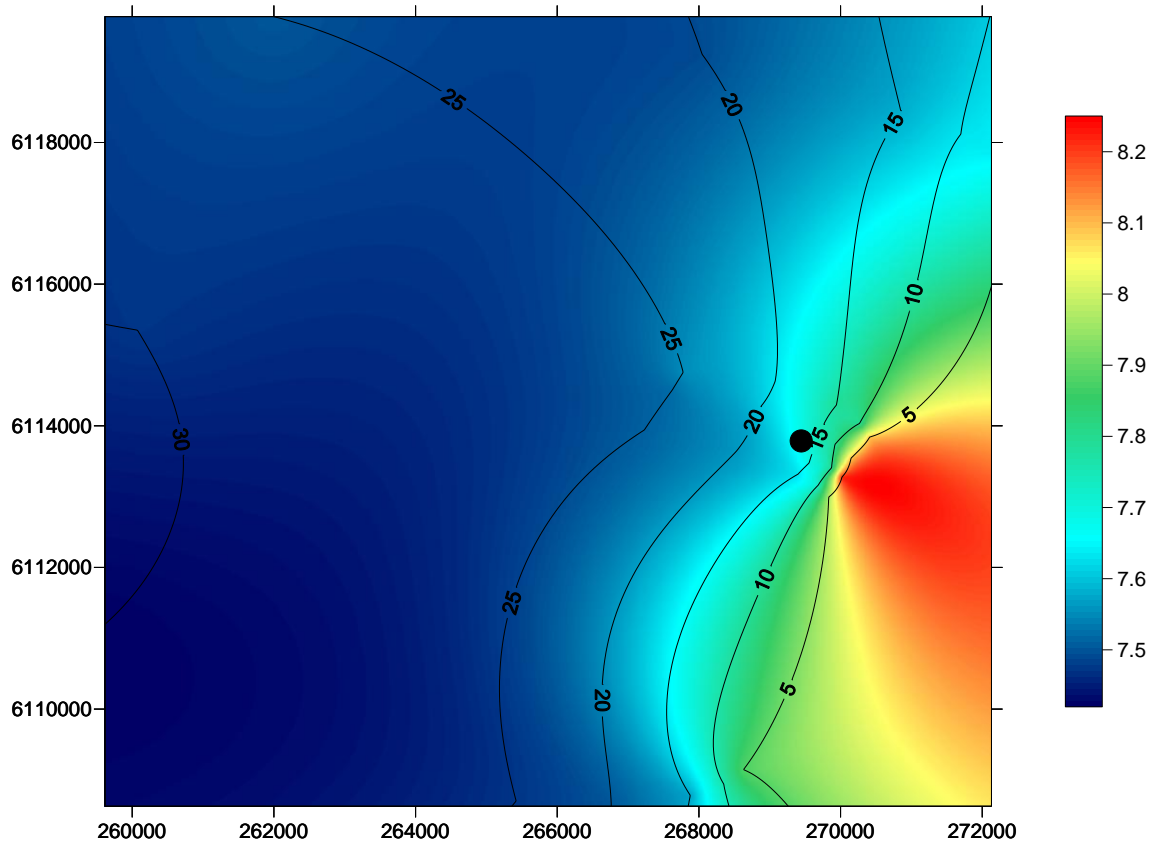
Figure 3 Spatial change in dissolved oxygen concentration, on the seafloor, in the Port Stanvac region. The coloured scale bar represents a change in the dissolved oxygen concentration between 7.4 mg/L and 8.2 mg/L. Contour lines denote a five metre change in depth. X coordinates refer to eastings and Y coordinates refer to northings measured in metres. Black dot represents position of ADP outfall. Water quality survey undertaken on the 4th June, 2010.
