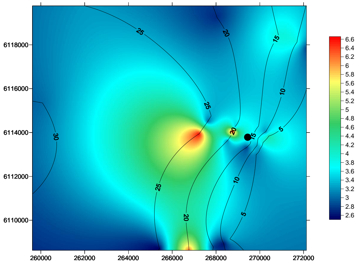
Figure 5 Spatial change in chlorophyll a concentration, one metre below the surface, in the Port Stanvac region. The coloured scale bar represents a change in chlorophyll concentration between 2.6 µg/L and 6.6 µg/L. Contour lines denote a five metre change in depth. X coordinates refer to eastings and Y coordinates refer to northings measured in metres. Black dot represents position of ADP outfall. Water quality survey undertaken on the 4th June, 2010.
