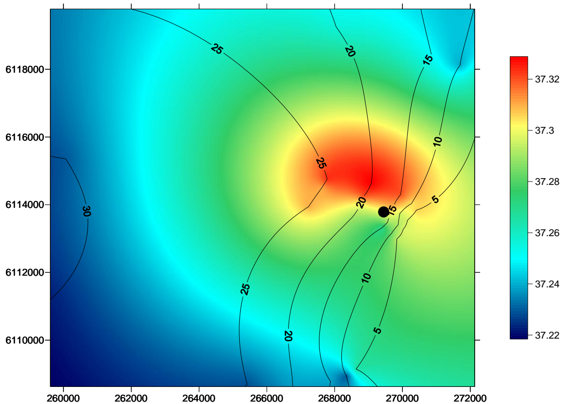
Figure 1 Spatial change in TDS (g/L) concentration, on the seafloor, in the Port Stanvac region. The coloured scale bar represents changes in TDS concentration between 37.2 g/L and 37.3 g/L. Contour lines denote a five metre change in depth. X coordinates refer to eastings and Y coordinates refer to northings measured in metres. Black dot represents position of ADP outfall. Water quality survey undertaken on the 4th June, 2010.
