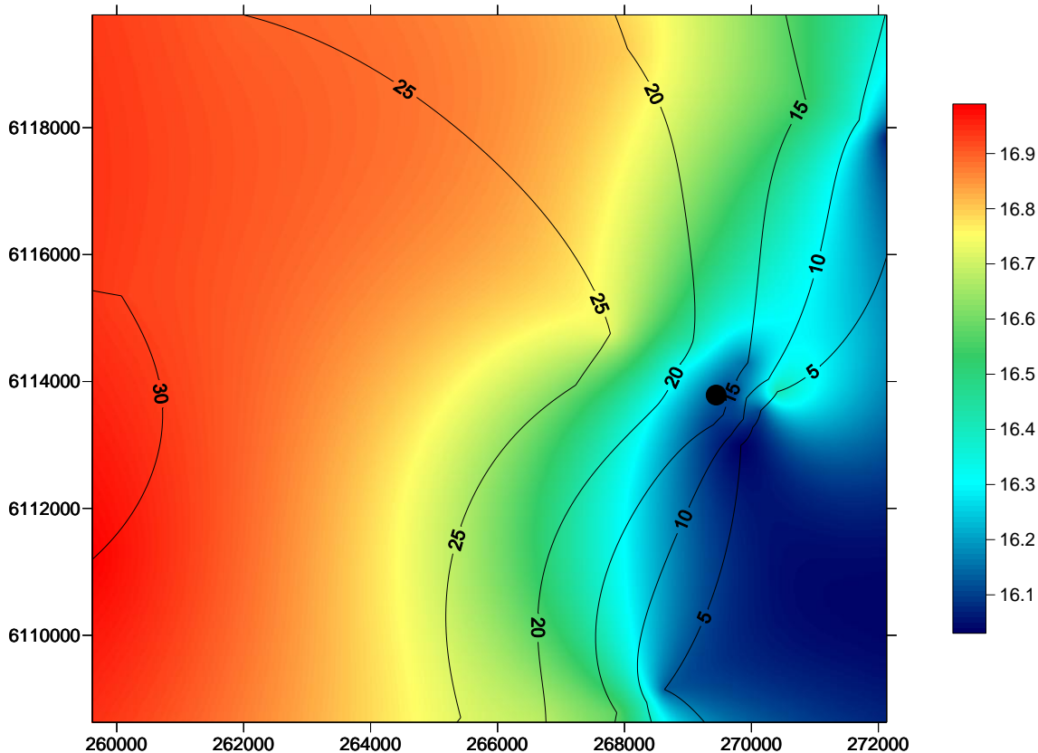
Figure 2 Spatial change in water temperature, on the seafloor, in the Port Stanvac region. The coloured scale bar represents temperature changes between 16.1 °C and 16.9 °C. Contour lines denote a five metre change in depth. X coordinates refer to eastings and Y coordinates refer to northings measured in metres. Black dot represents position of ADP outfall. Water quality survey undertaken on the 4th June, 2010.
