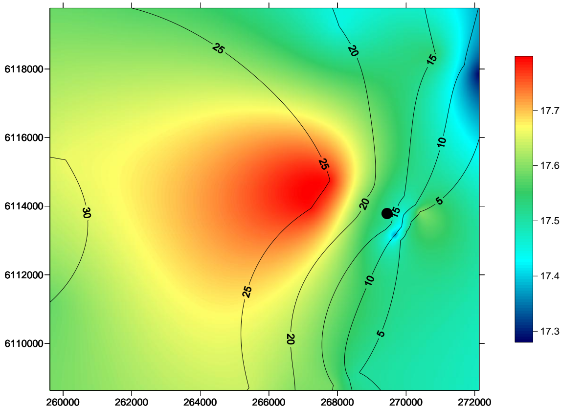
Figure 2 Spatial change in water temperature, on the seafloor, in the Port Stanvac region. The coloured scale bar represents temperature changes between 17.3 °C and 17.7 °C. Contour lines denote a five metre change in depth. X coordinates refer to eastings and Y coordinates refer to northings measured in metres. Black dot represents position of ADP outfall. Water quality survey undertaken on the 18th May, 2010.
