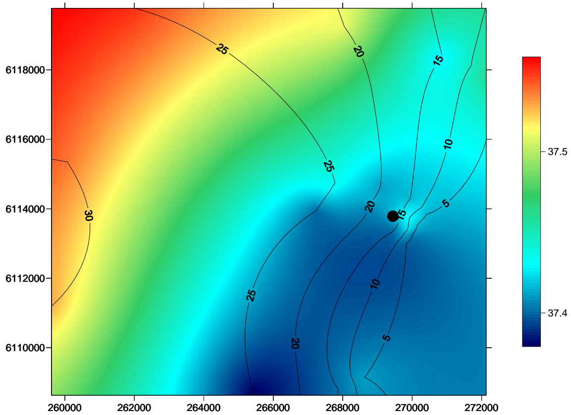
Figure 1 Spatial change in TDS (g/L) concentration, on the seafloor, in the Port Stanvac region. The coloured scale bar represents changes in TDS concentration between 37.3 g/L and 37.6 g/L. Contour lines denote a five metre change in depth. X coordinates refer to eastings and Y coordinates refer to northings measured in metres. Black dot represents position of ADP outfall. Water quality survey undertaken on the 18th May, 2010.
