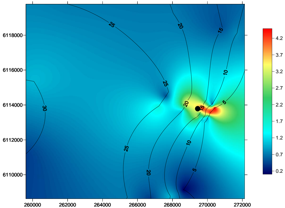
Figure 5 Spatial change in chlorophyll a concentration, one metre below the surface, in the Port Stanvac region. The coloured scale bar represents a change in chlorophyll concentration between 0.2 µg/L and 4.2 µg/L. Note sensor sensitivity is \pm 1 µg/L. Contour lines denote a five metre change in depth. The bottom scale bar represents distance in metres across the region. X coordinates refer to eastings and Y coordinates refer to northings measured in metres. Black dot represents position of ADP outfall.
