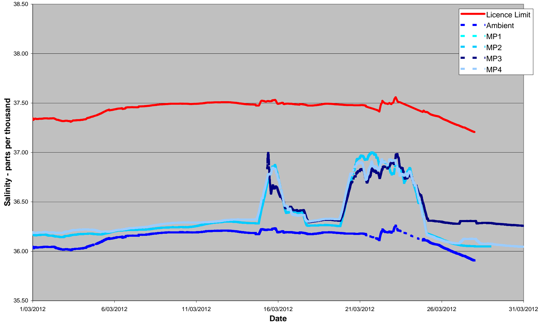
March 2012 24 Hour Average Salinity at 100 metres from Diffuser
