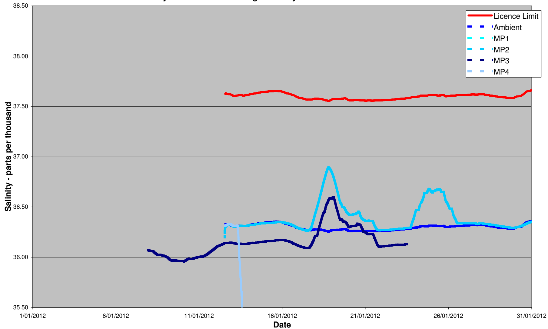
January 2012 24 Hour Average Salinity at 100 metres from Diffuser
