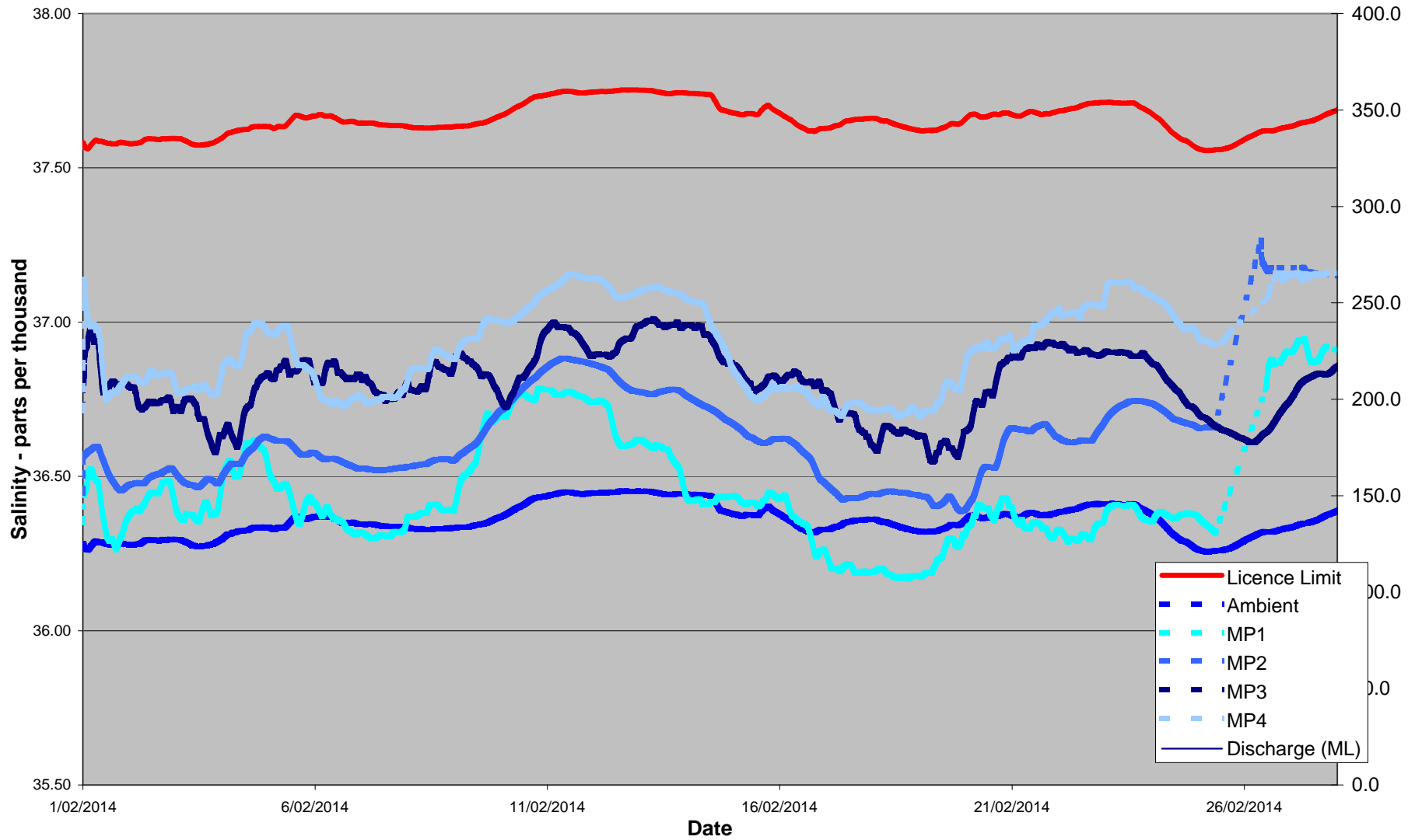
February 2014 24 Hour Average Salinity at 100 metres from Diffuser
