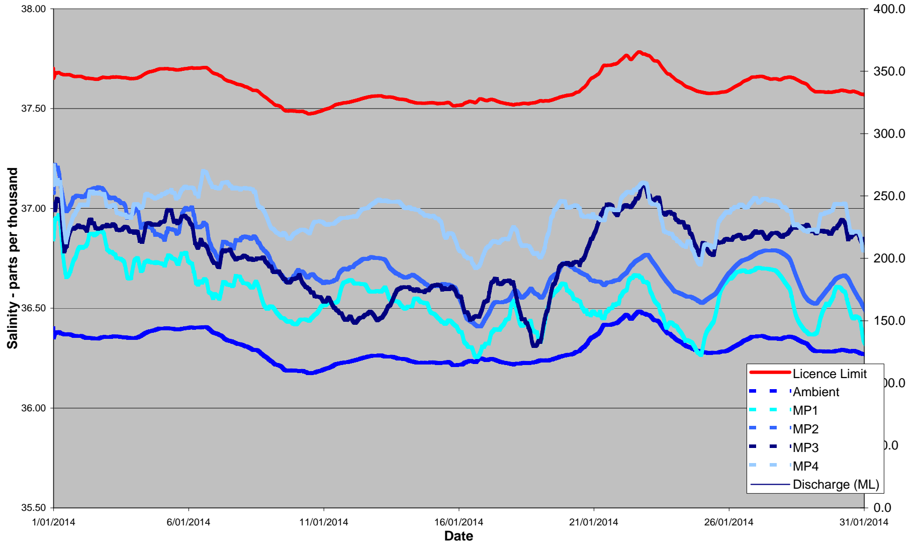
January 2014 24 Hour Average Salinity at 100 metres from Diffuser
