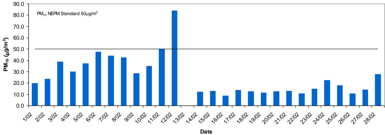
Le Fevre 1 Daily Average PM10 - February 2014
