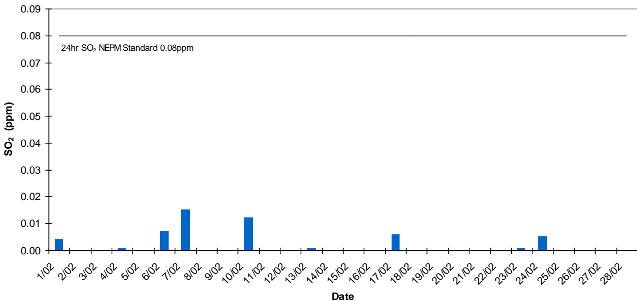
Pt Pirie Daily Average SO2 - February 2014
