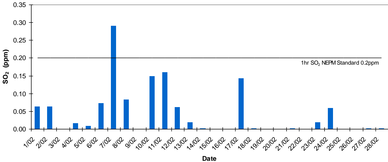
Pt Pirie 1 Hr Daily Maxima SO2 February 2014
