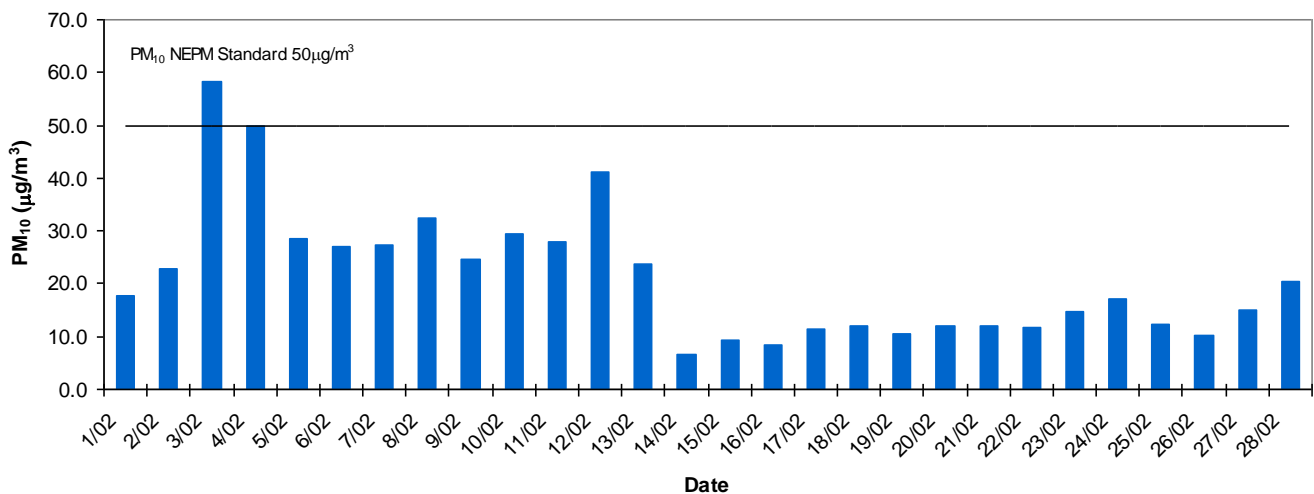
Southern Adelaide Daily Average PM10 - February 2014
