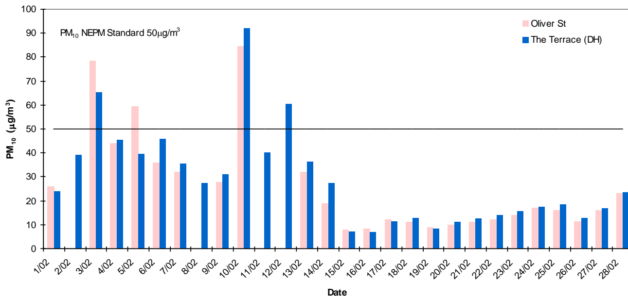
Pt Pirie Daily Average PM10 - February 2014
