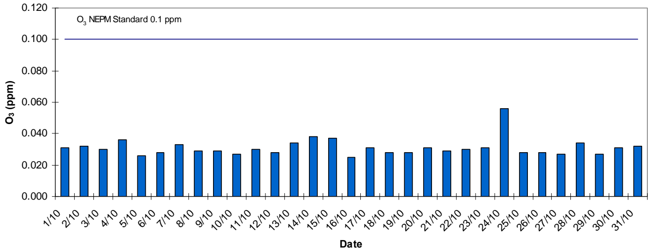
North eastern Adelaide 1 Hr Daily Maxima O3 - October 2012
