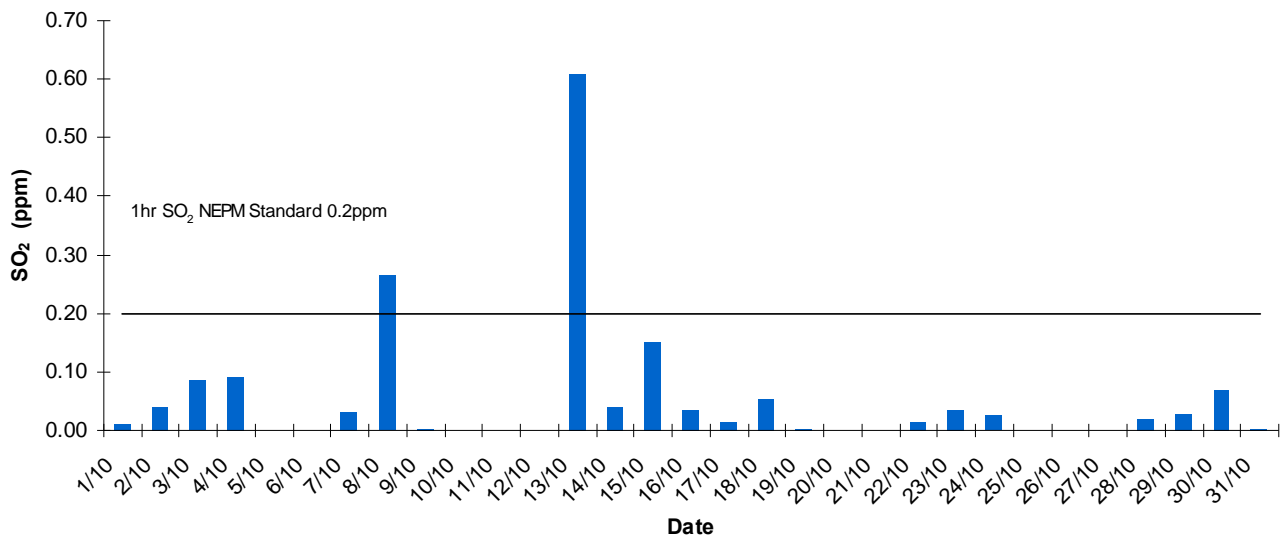
Pt Pirie 1 Hr Daily Maxima SO2 October 2012
