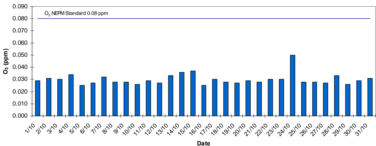
North eastern Adelaide 4 Hr Daily Maxima O3 October 2012
