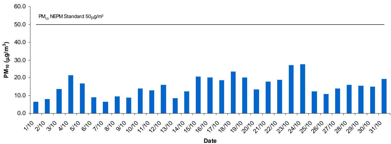
Southern Adelaide Daily Average PM10 - October 2012
