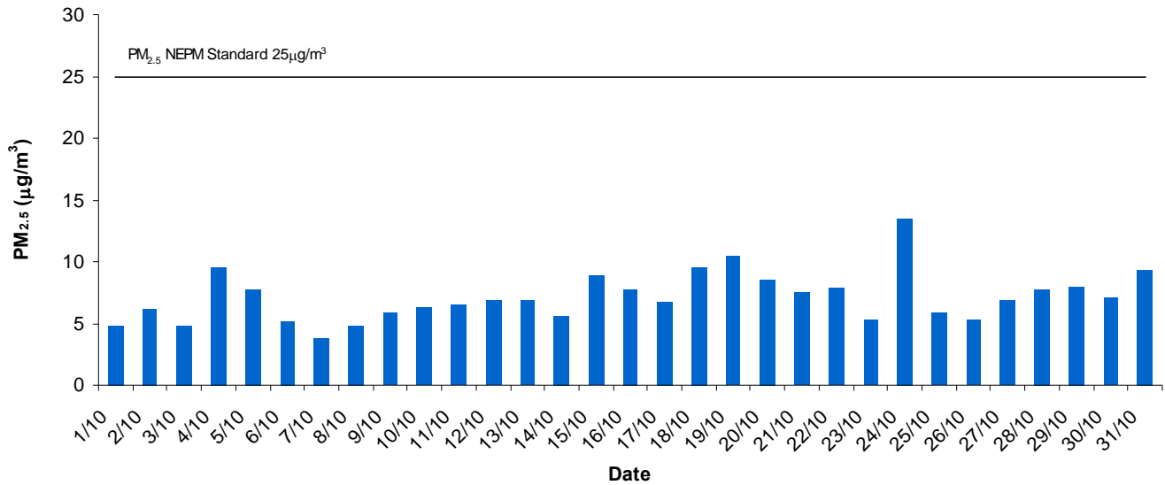
Western Adelaide Daily Average PM2.5 - October 2012
