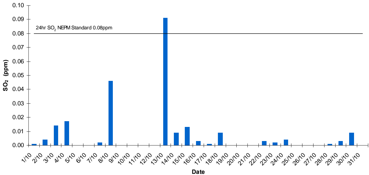
Pt Pirie Daily Average SO2 - October 2012
