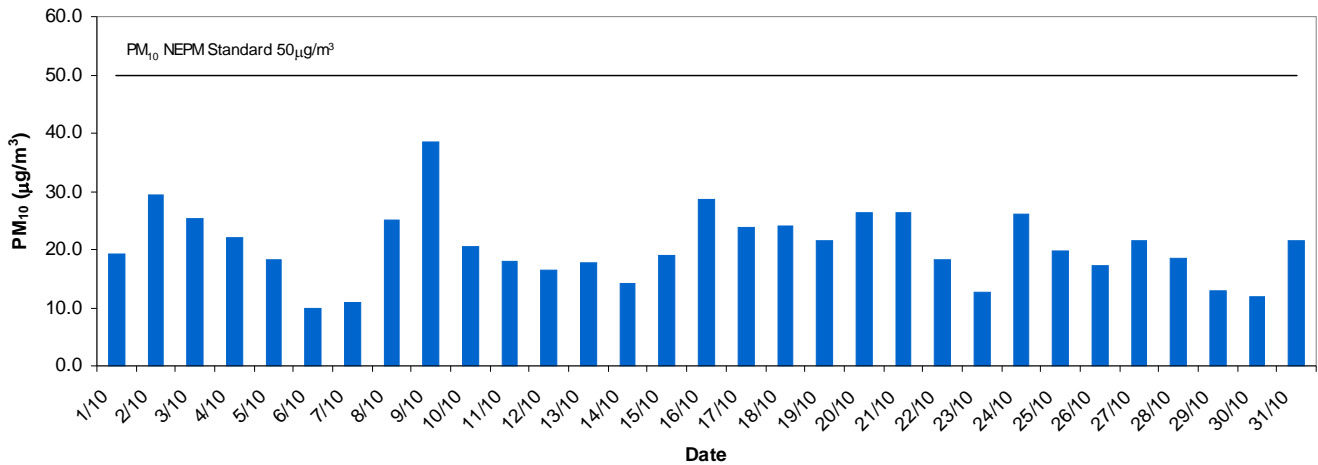
Le Fevre 1 Daily Average PM10 - October 2013
