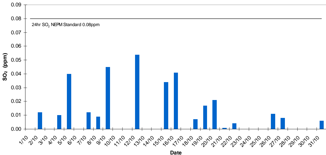
Pt Pirie Daily Average SO 2 - October 2013
