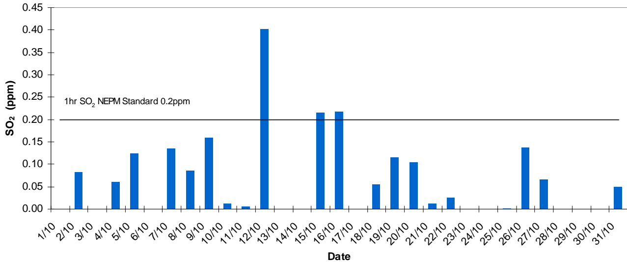
Pt Pirie 1 Hr Daily Maxima SO 2 October 2013
