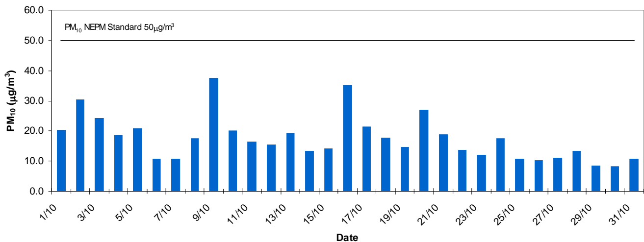
Southern Adelaide Daily Average PM10 - October 2013
