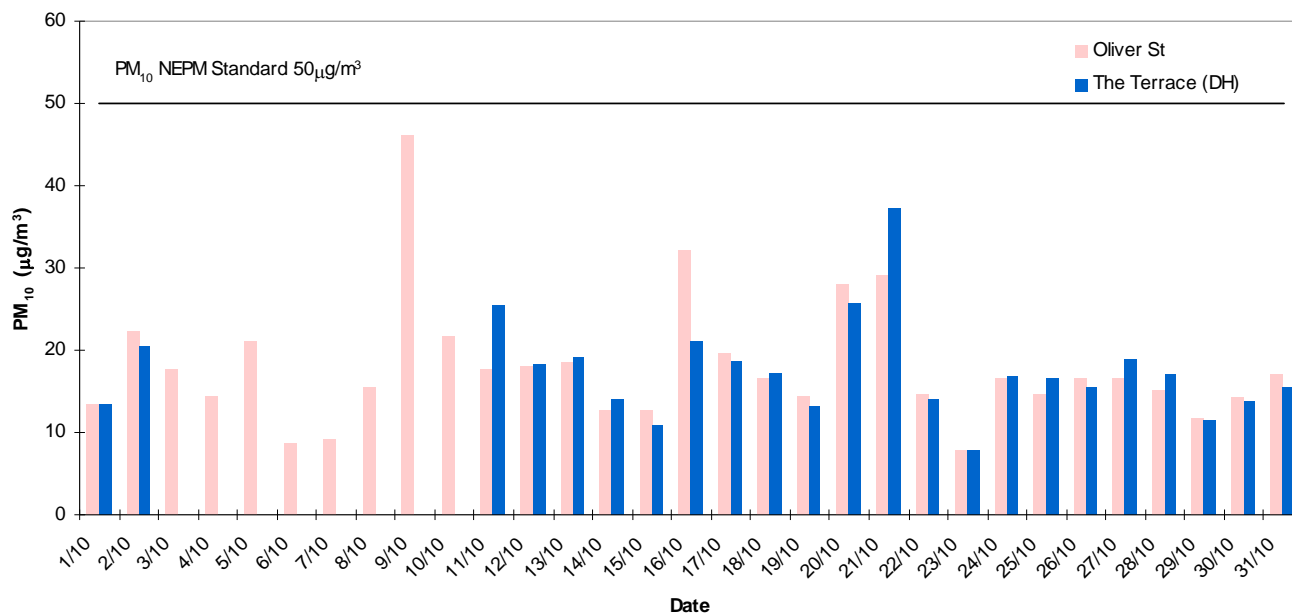
Pt Pirie Daily Average PM10 - October 2013
