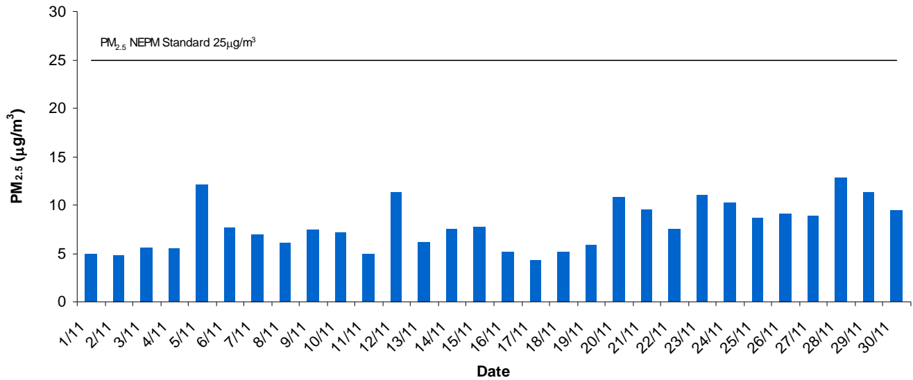
Western Adelaide Daily Average PM 2.5 - November 2012
