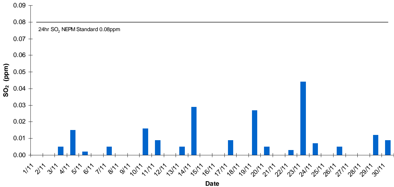
Pt Pirie Daily Average SO2 - November 2012
