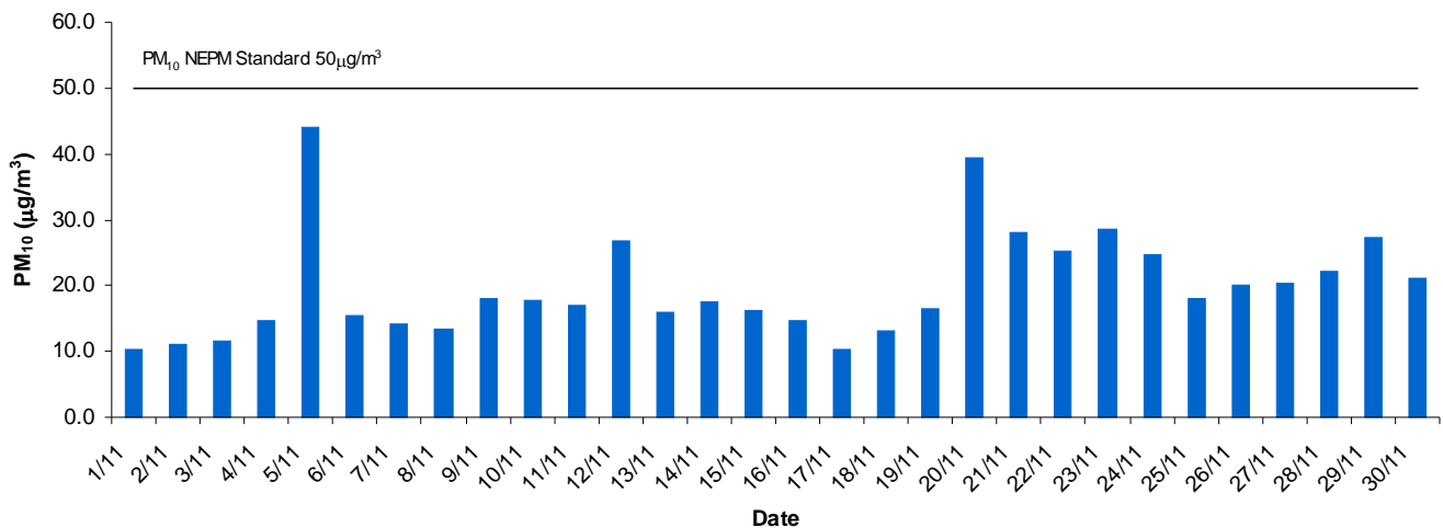
Southern Adelaide Daily Average PM10 - November 2012
