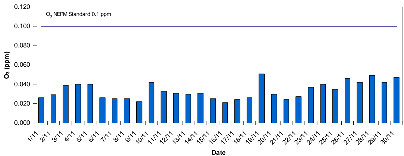
Western Adelaide 1 Hr Daily Maxima O 3 - November 2012
