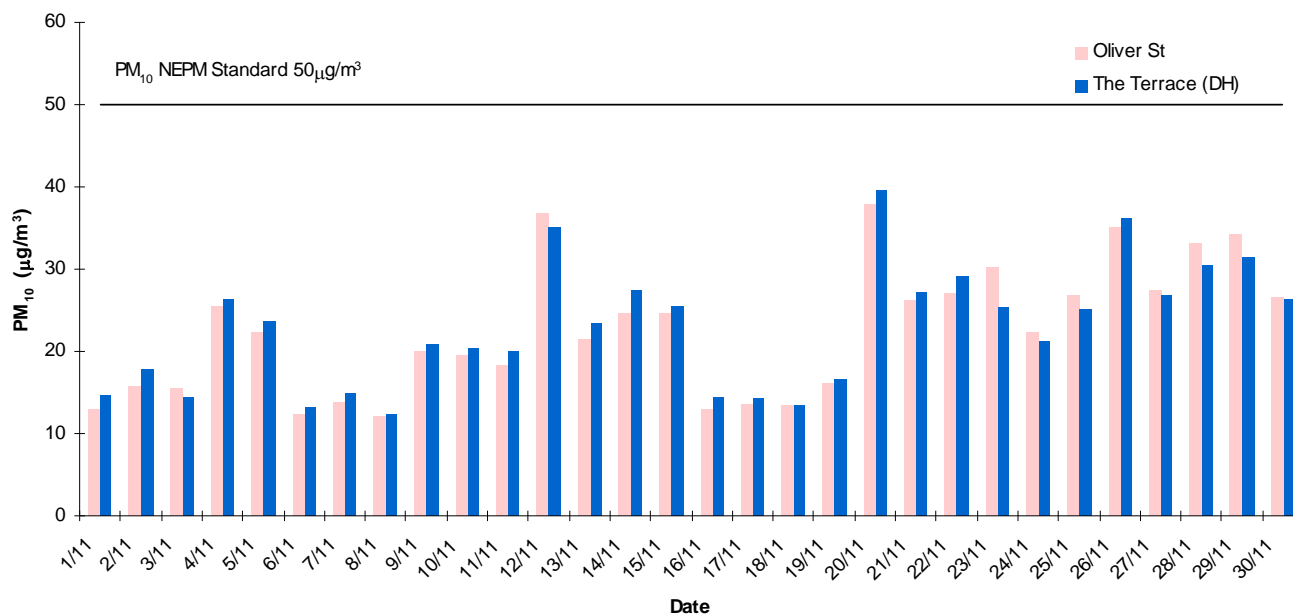
Pt Pirie Daily Average PM10 - November 2012
