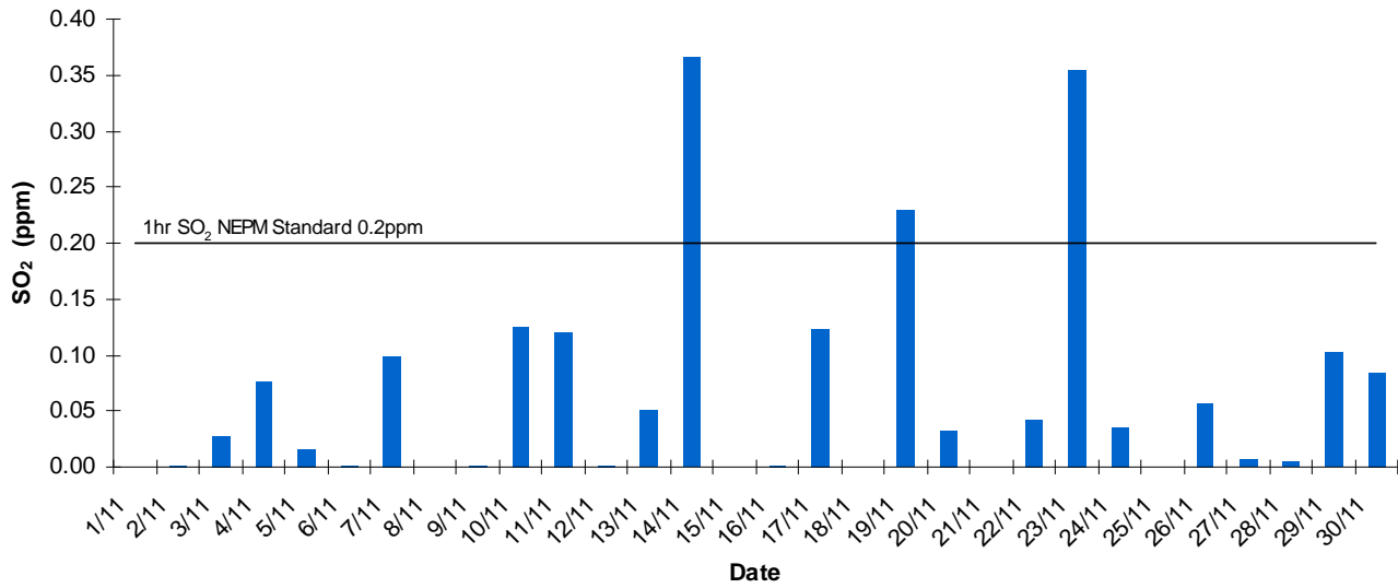
Pt Pirie 1 Hr Daily Maxima SO2 November 2012
