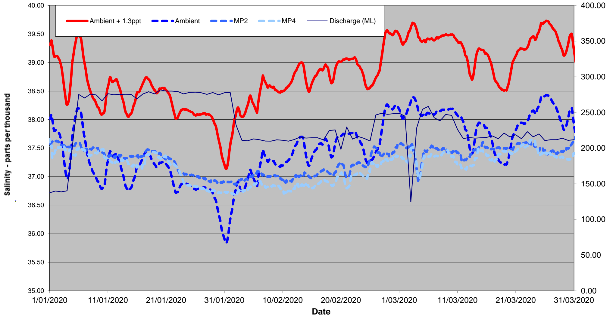
January to March 2020 24 Hour Average Salinity at 100 metres from Diffuser
