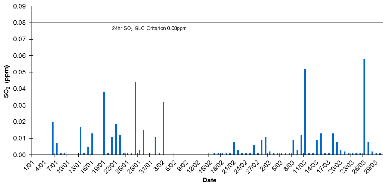
Pt Pirie Daily Average SO 2 - Quarter 1, 2017
