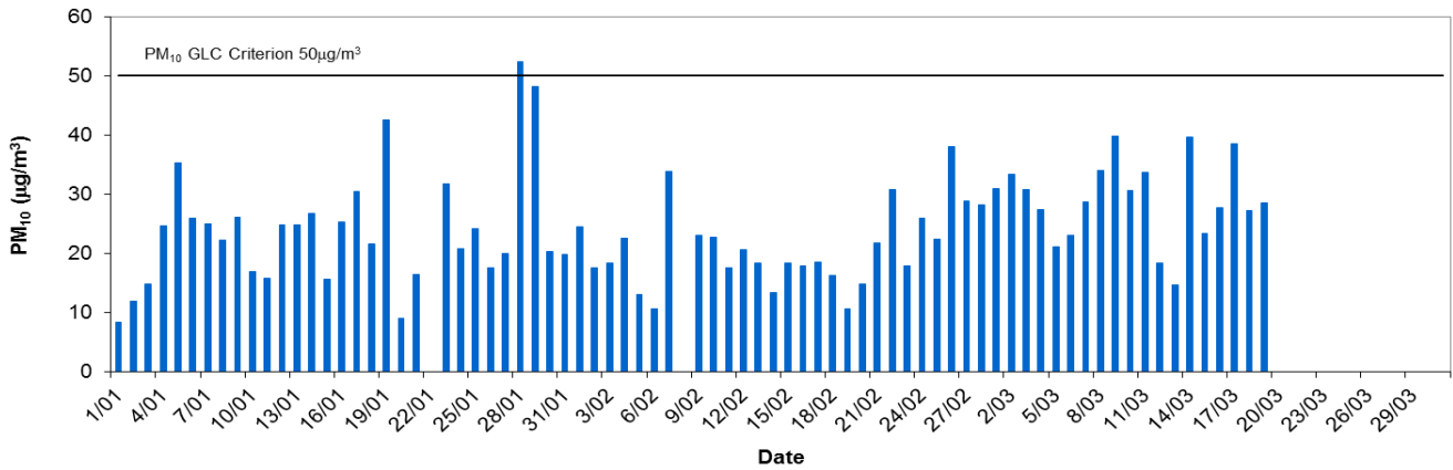
Le Fevre 2 Daily Average PM10 - Quarter 1, 2017
