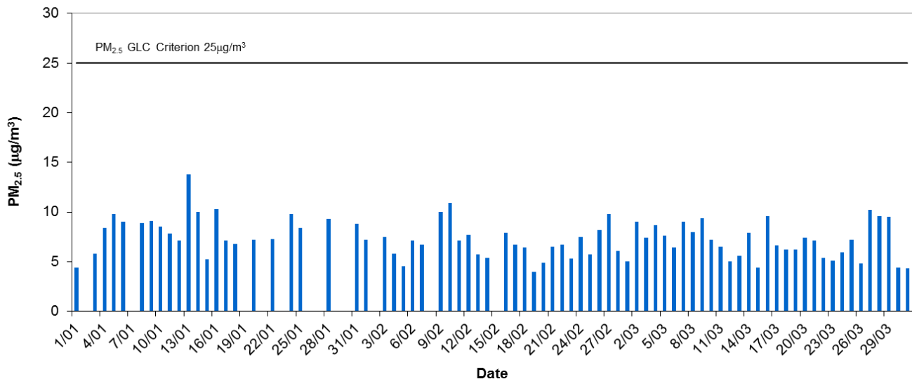
Adelaide CBD Daily Average PM 2.5 - Quarter 1, 2017
