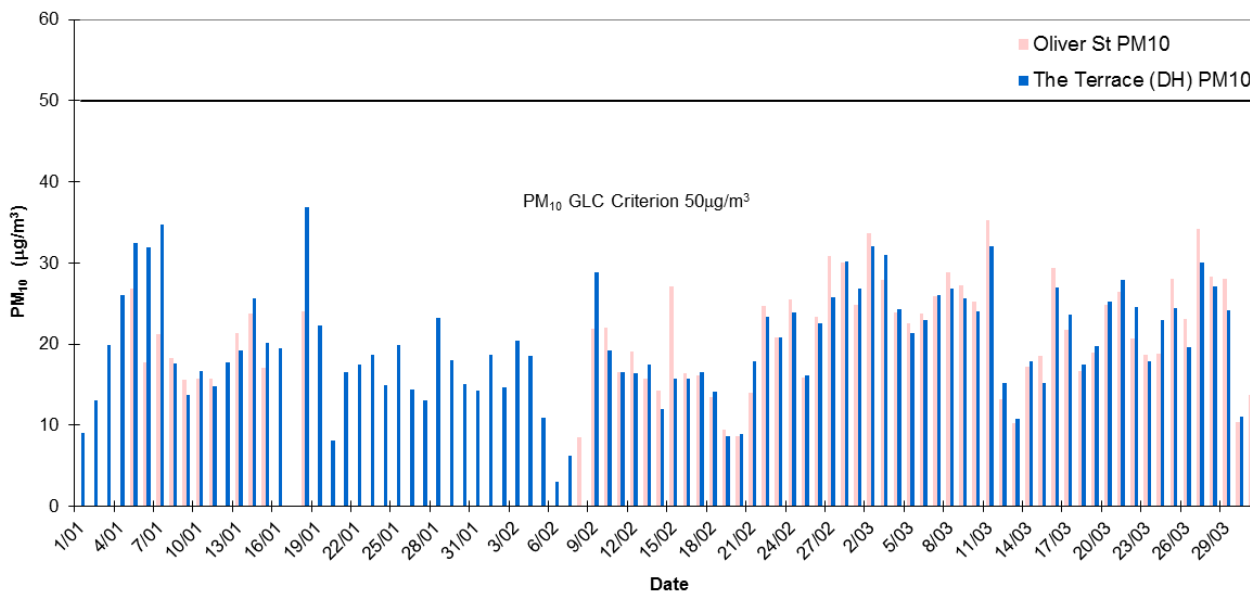
Pt Pirie Daily Average PM 10 - Quarter 1, 2017
