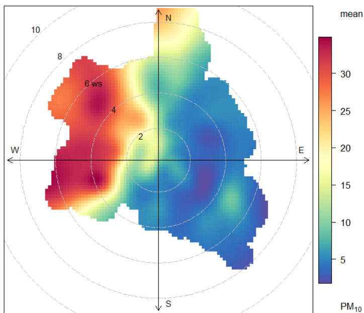
Polar Plot for PM 10 (10-minute averaged data in \mu\text{g}/\text{m}^3 ) August 2016
