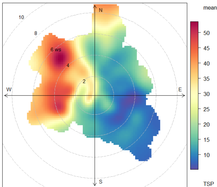
Polar Plot for TSP (10-minute averaged data in \mu\text{g}/\text{m}^3 ) August 2016
