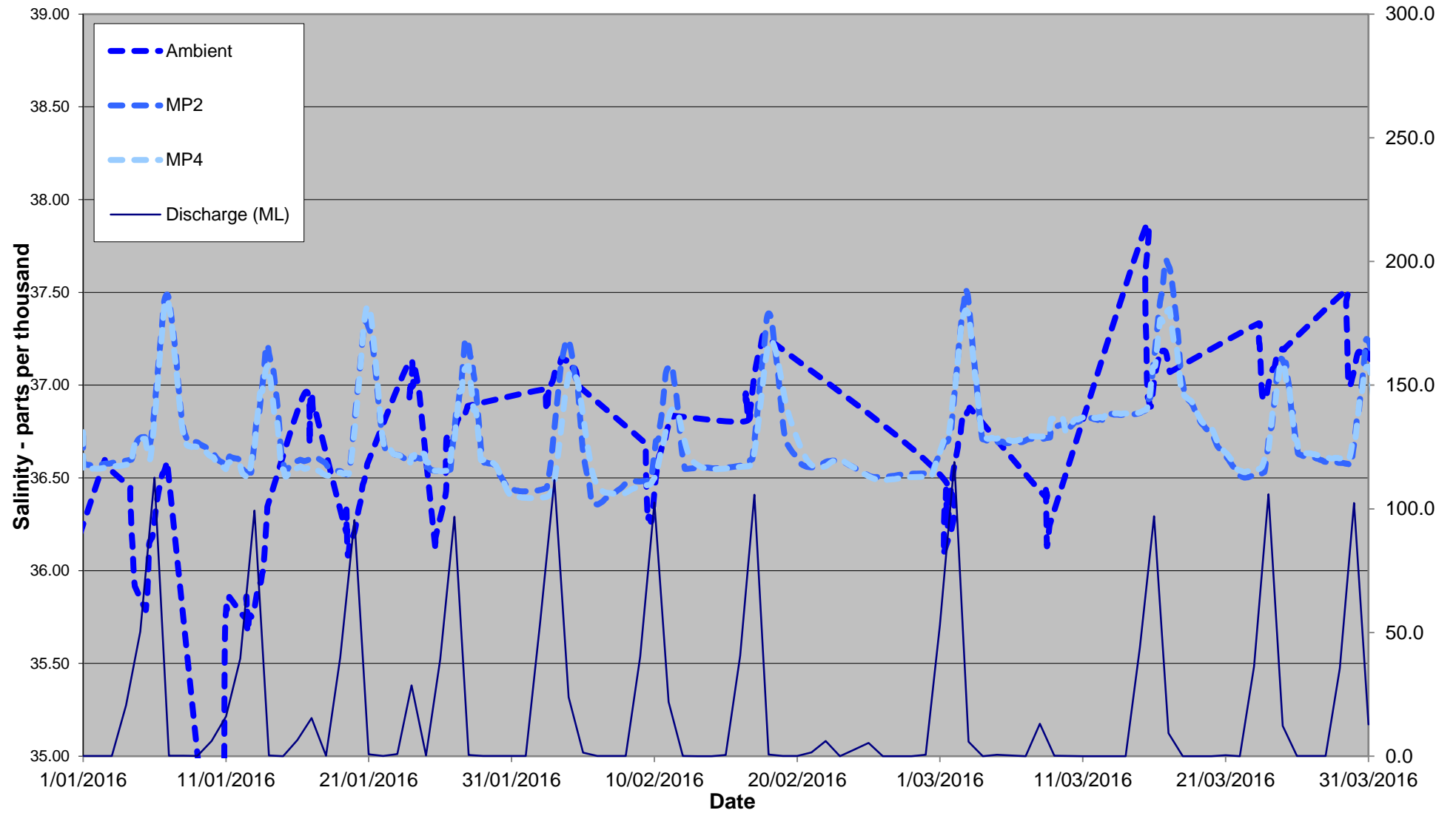
January to March 2016 24 Hour Average Salinity at 100 metres from Diffuser
