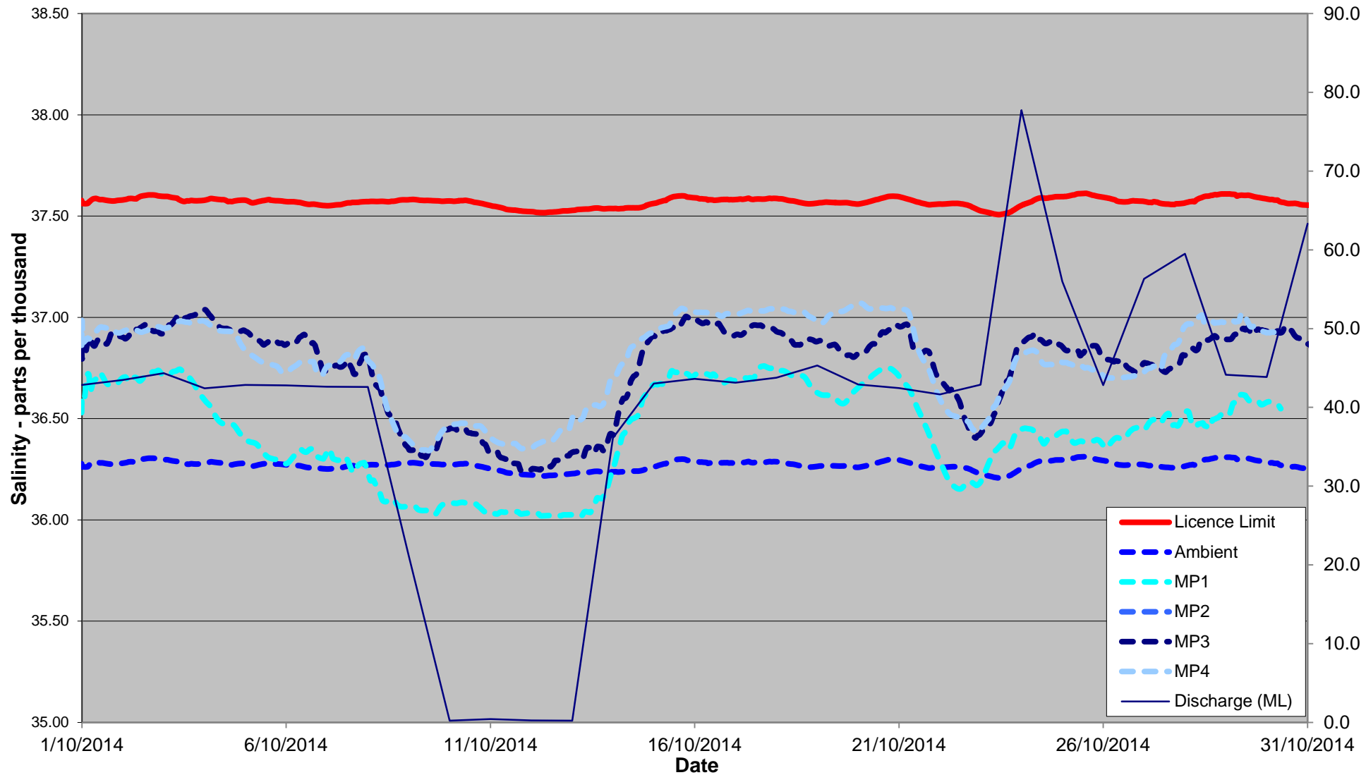
October 2014 24 Hour Average Salinity at 100 metres from Diffuser
