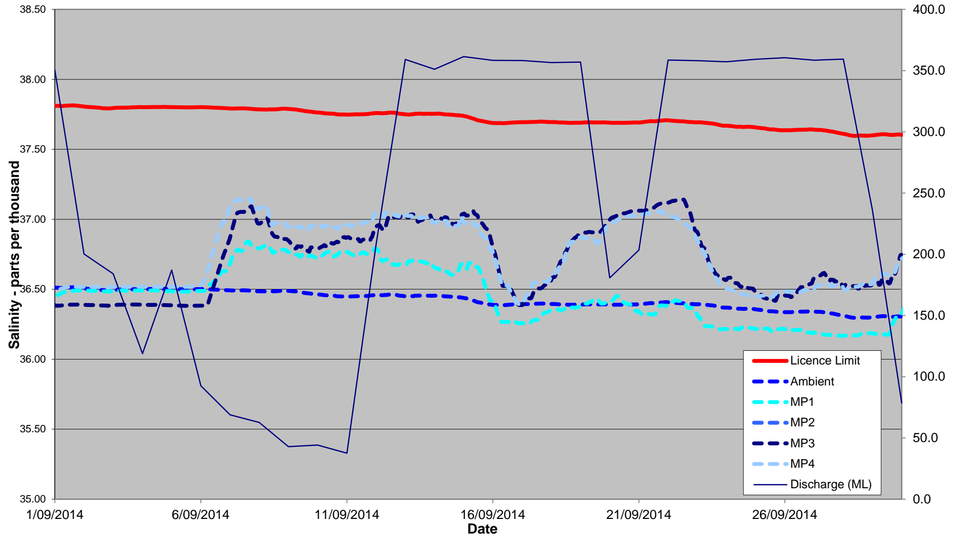
September 2014 24 Hour Average Salinity at 100 metres from Diffuser
