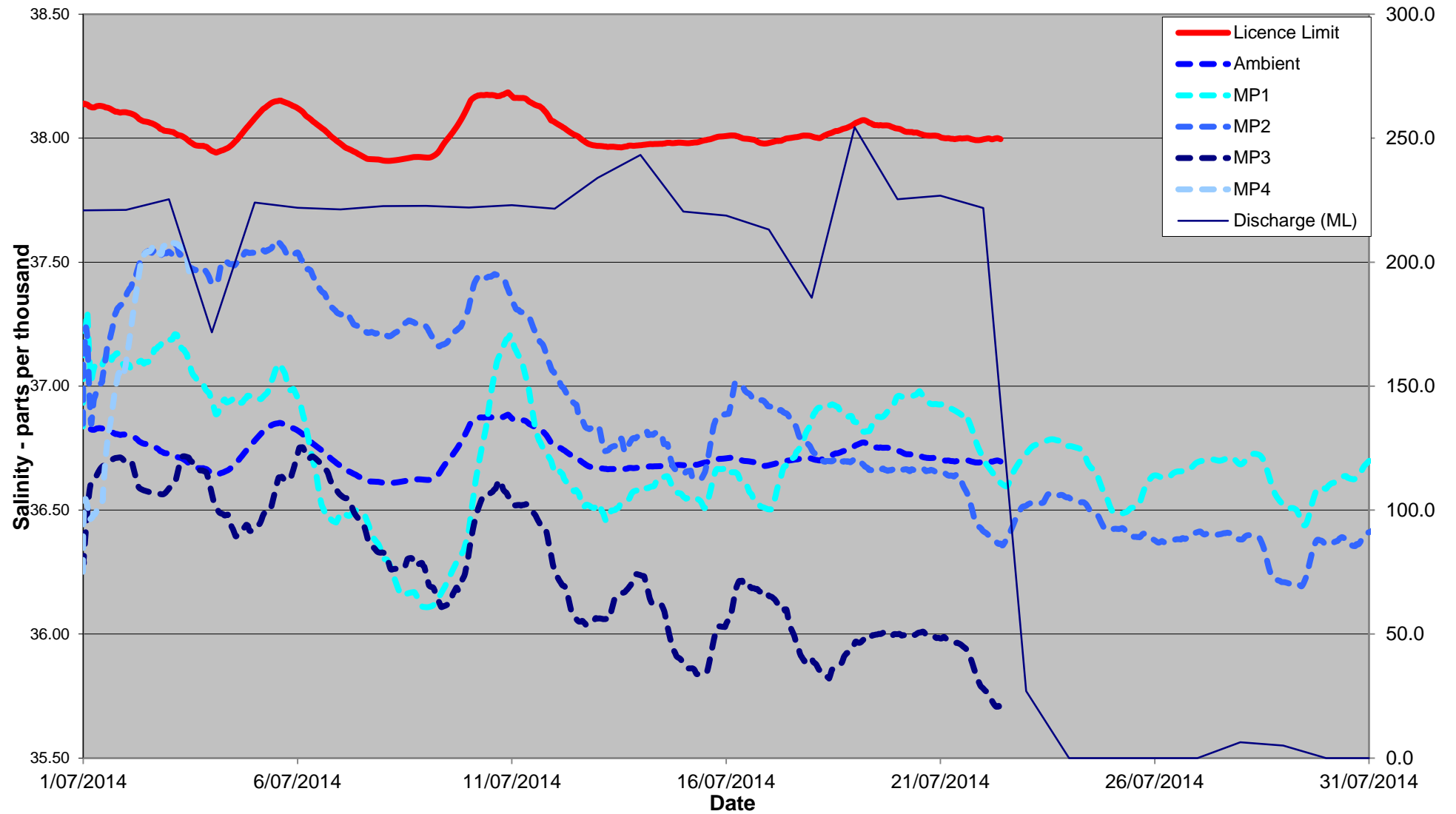
July 2014 24 Hour Average Salinity at 100 metres from Diffuser
