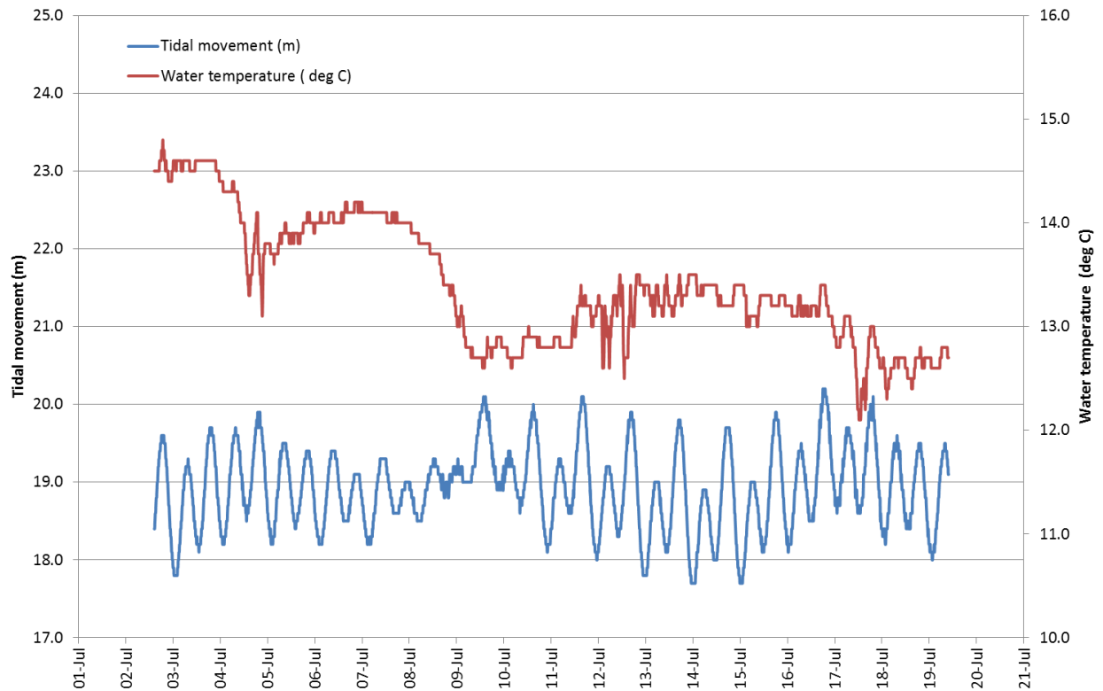
Figure 5. Changes in dissolved temperature (°C) with tidal movement (m) over 18 days, 2 nd July to the 19 th July 2014.
