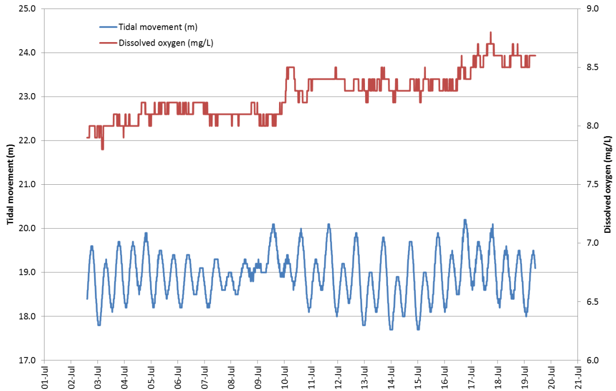
Figure 3. Changes in dissolved oxygen (mg/L) with tidal movement (m) over 18 days, 2 nd July to the 19 th July 2014.
