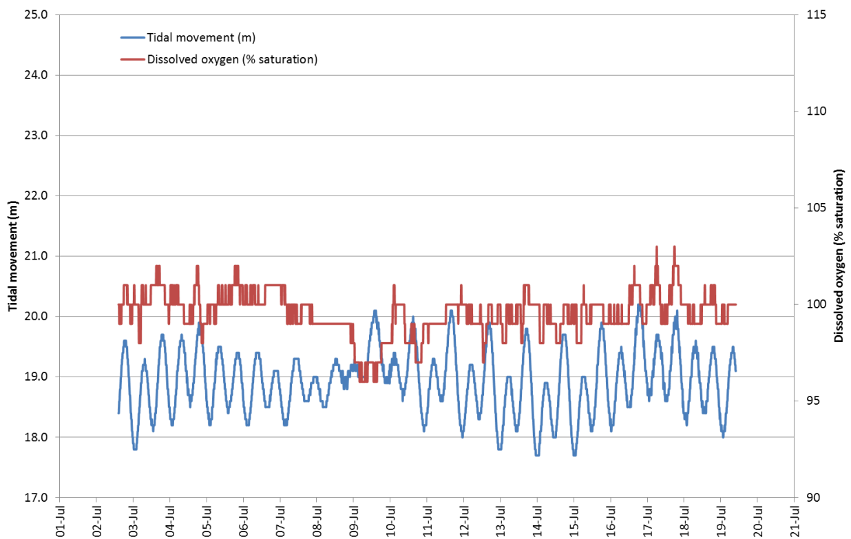
Figure 2. Changes in dissolved oxygen (%) with tidal movement (m) over 18 days, 2 nd July to the 19 th July 2014.
