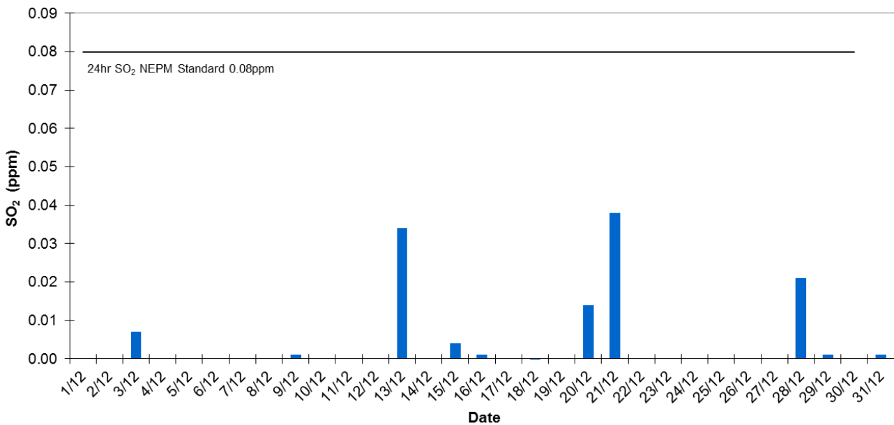
Pt Pirie Daily Average SO2 - December 2014
