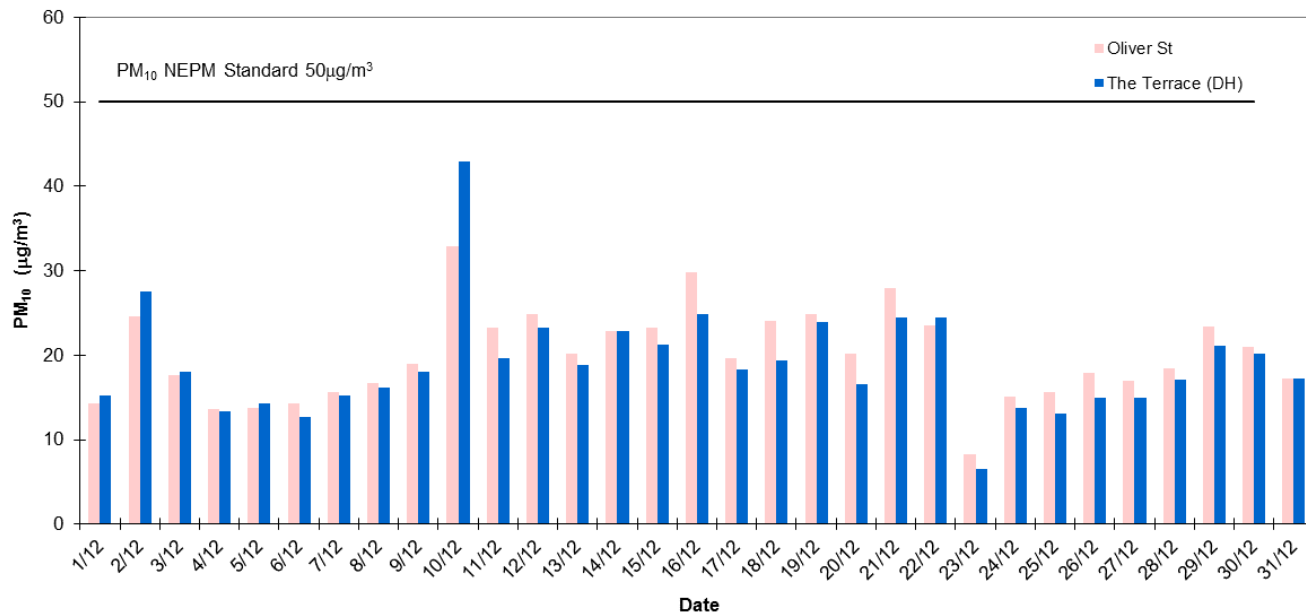
Pt Pirie Daily Average PM 10 - December 2014
