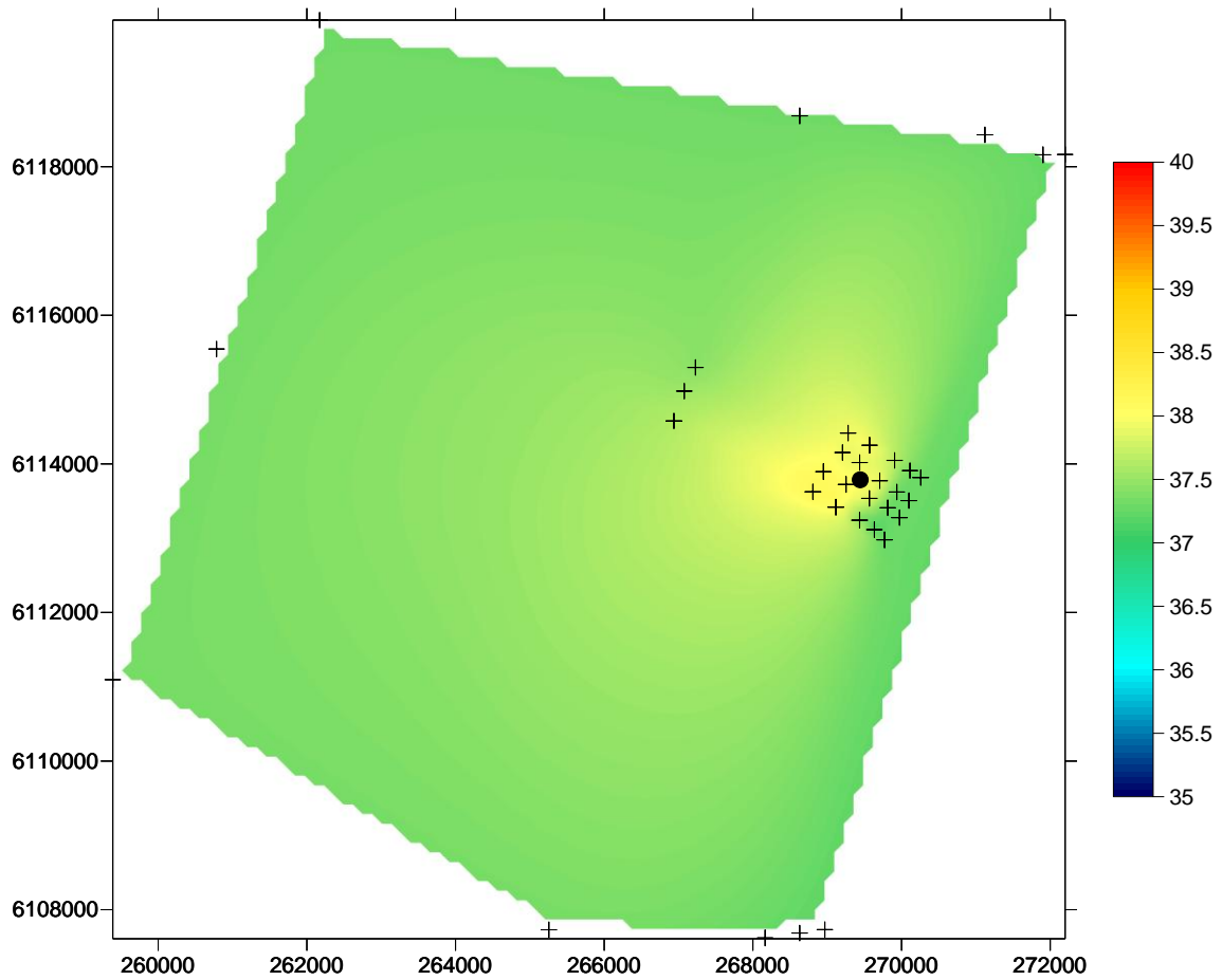
Figure 2 Spatial change in salinity concentration (parts per thousand), on the seafloor, in the Port Stanvac region. The coloured scale bar represents changes in salinity concentration between 35 ppt and 40 ppt (sensor error \pm 0.1 ppt). X coordinates refer to eastings and Y coordinates refer to northings measured in metres. Black dot represents position of ADP outfall. Black crosses represent water quality sampling locations (also refer to Figure 1).
