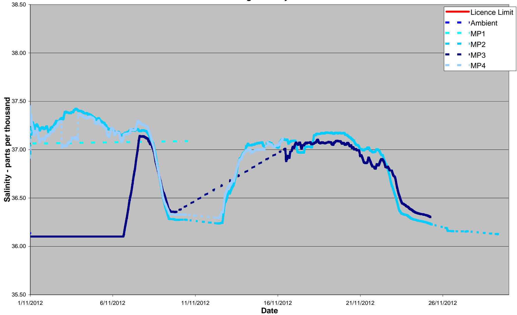
November 2012 24 Hour Average Salinity at 100 metres from Diffuser
