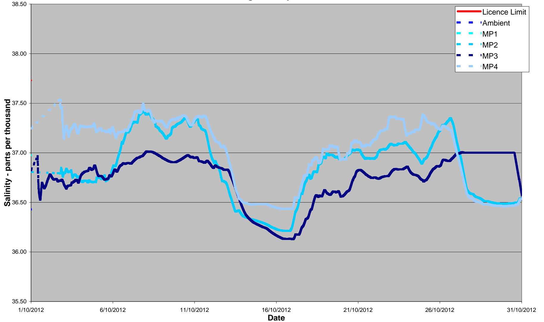
October 2012 24 Hour Average Salinity at 100 metres from Diffuser
