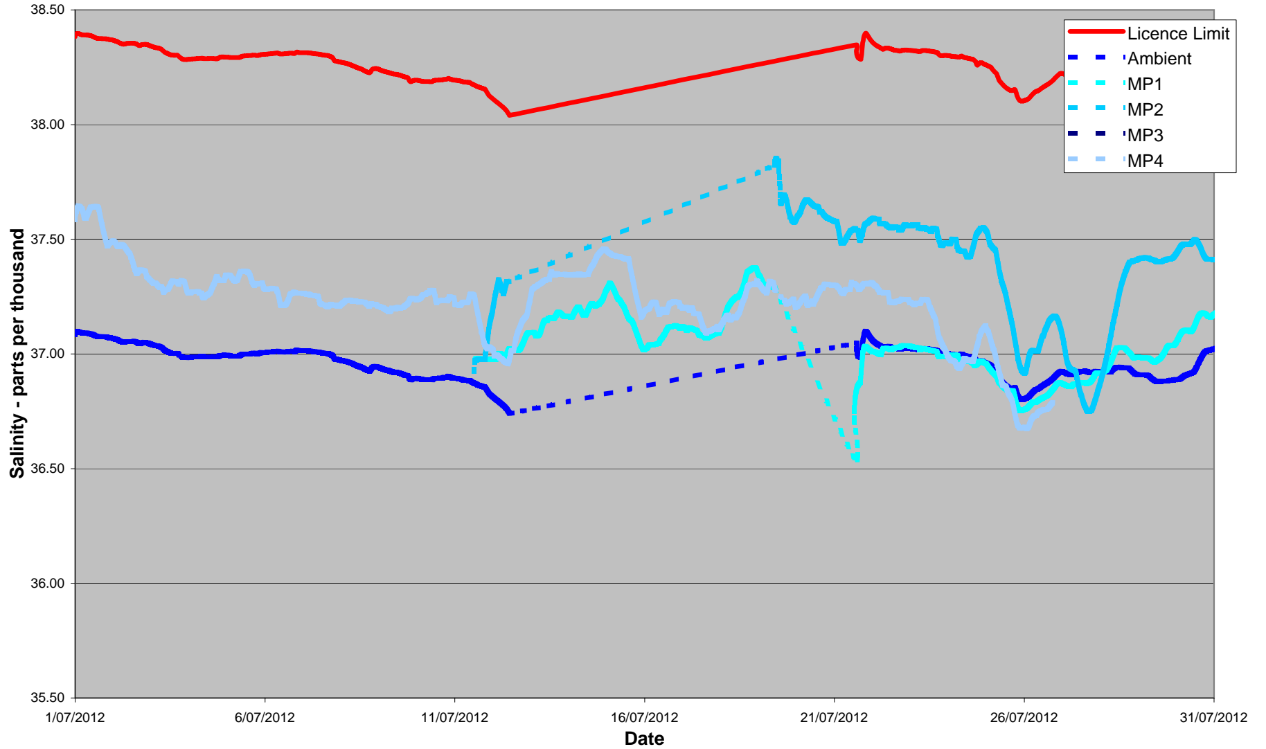
July 2012 24 Hour Average Salinity at 100 metres from Diffuser
