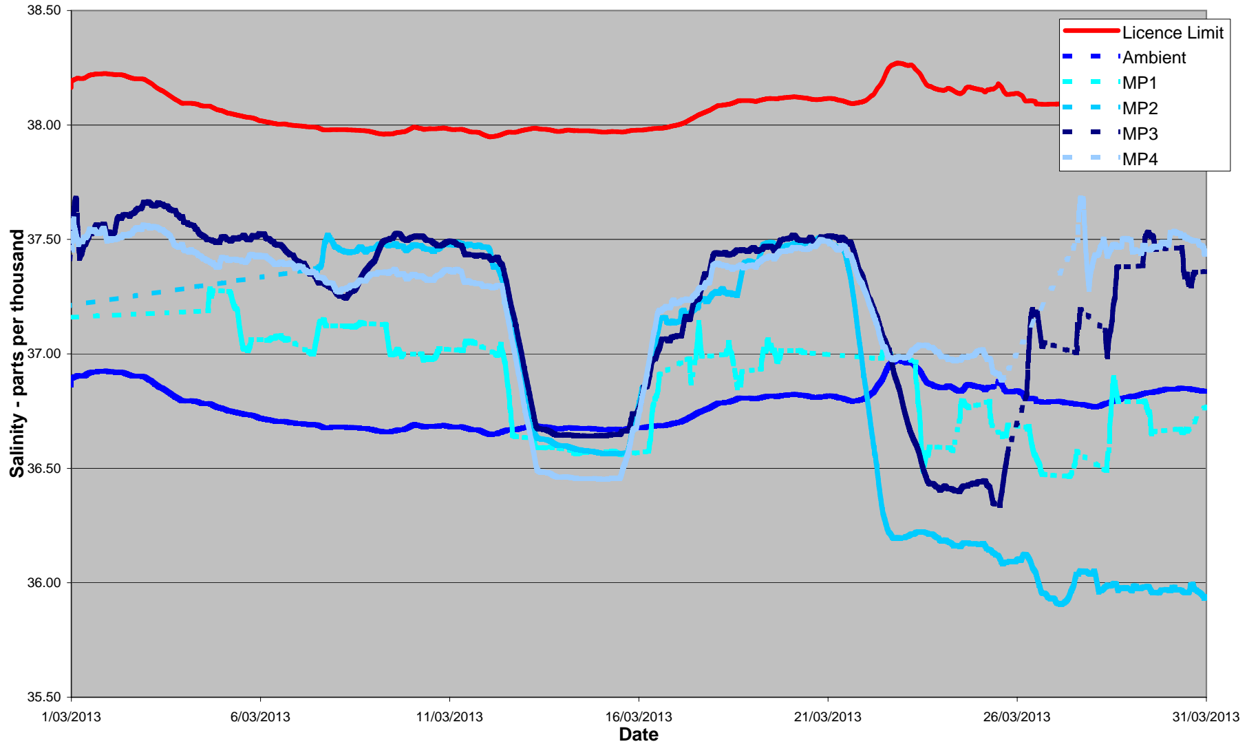
March 2013 24 Hour Average Salinity at 100 metres from Diffuser
