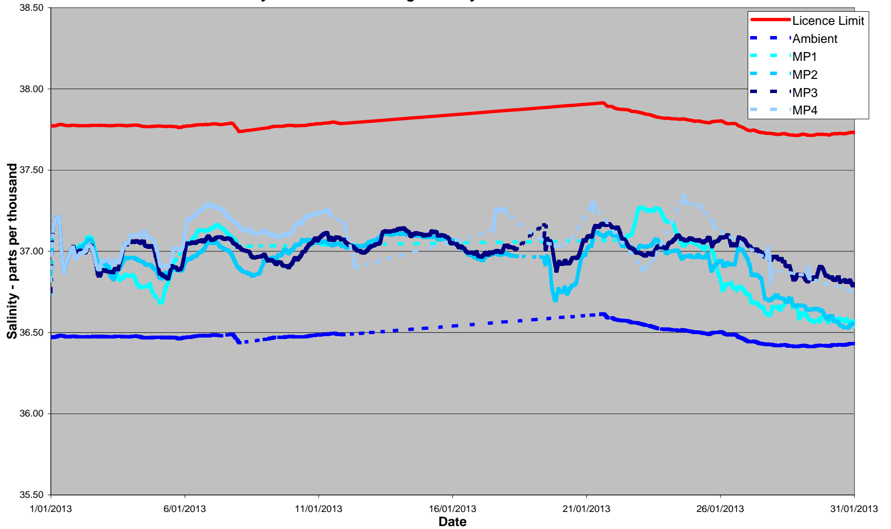
January 2013 24 Hour Average Salinity at 100 metres from Diffuser
