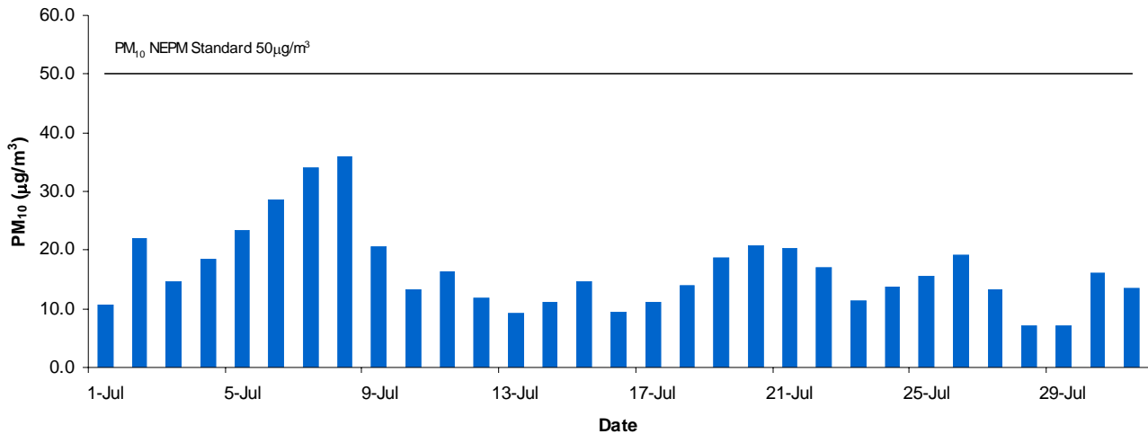
North western Adelaide Daily Average PM10 - July 2012
