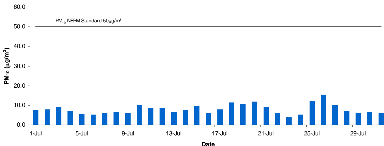
Eastern Adelaide Daily Average PM10 - July 2012
