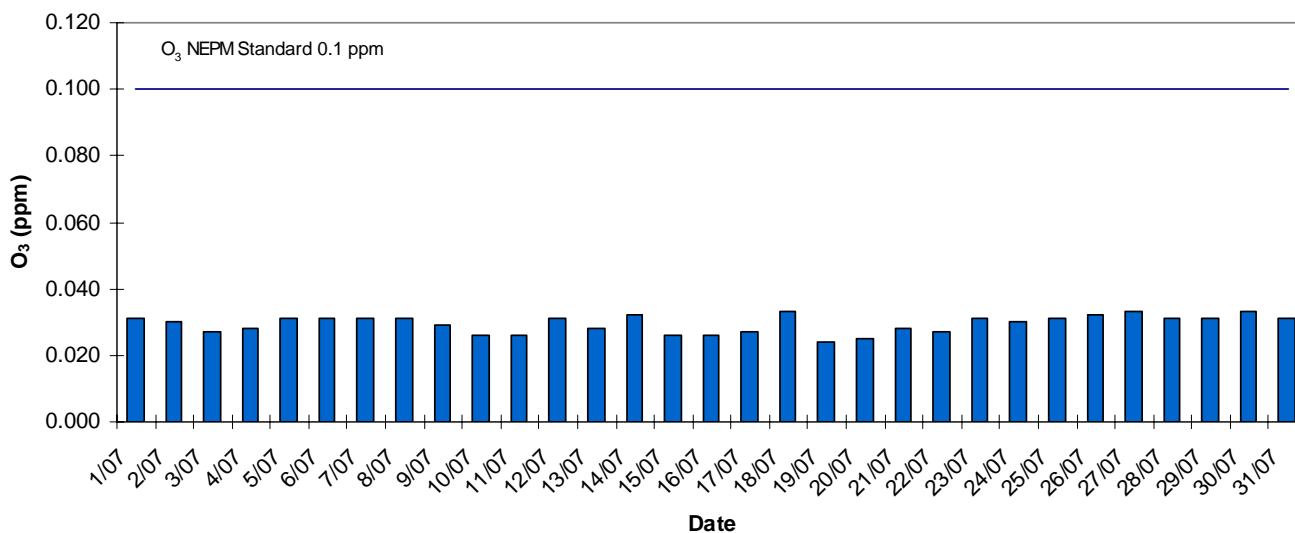
Eastern Adelaide 1 Hr Daily Maxima O3 - July 2012
