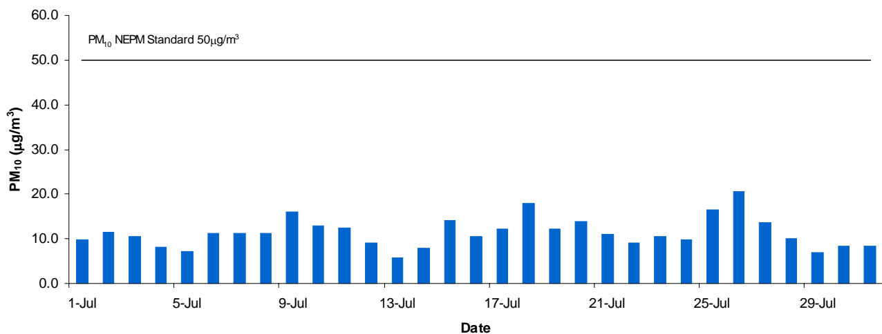
Southern Adelaide Daily Average PM10 - July 2012
