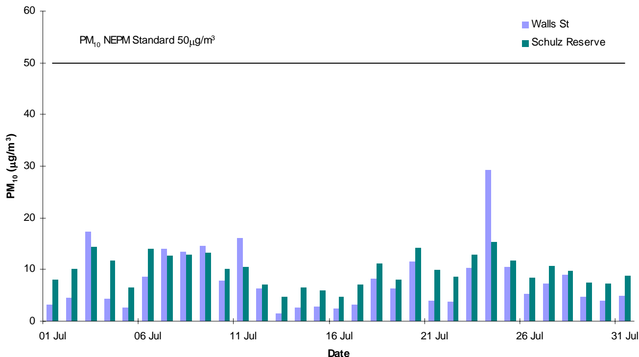
Whyalla Daily Average PM10 - July 2012
