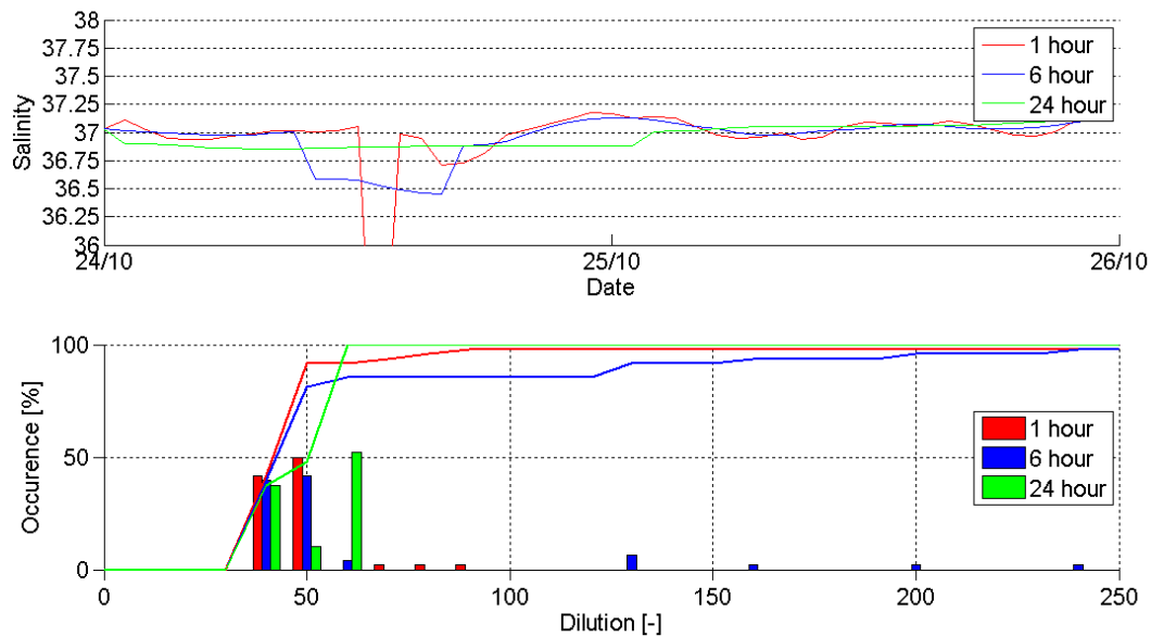
Figure 3 Measured Offshore Arc 1, Salinity and Dilution Values during the Dodge Tide (24/10/2012 – 26/10/2012)
