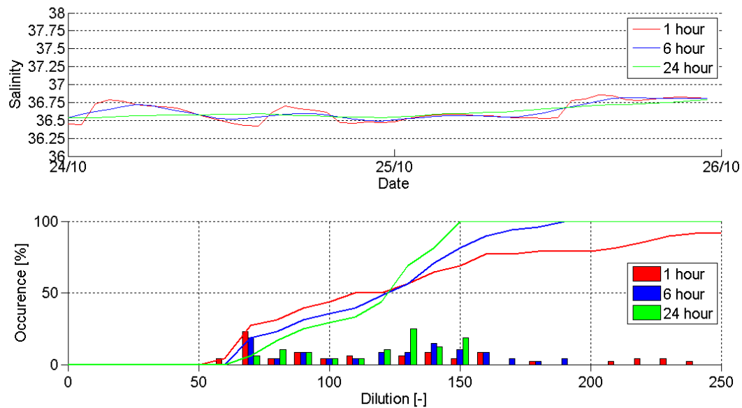
Figure 5 Measured Offshore Arc 2, Salinity and Dilution Values during the Dodge Tide (24/10/2012 – 26/10/2012)
