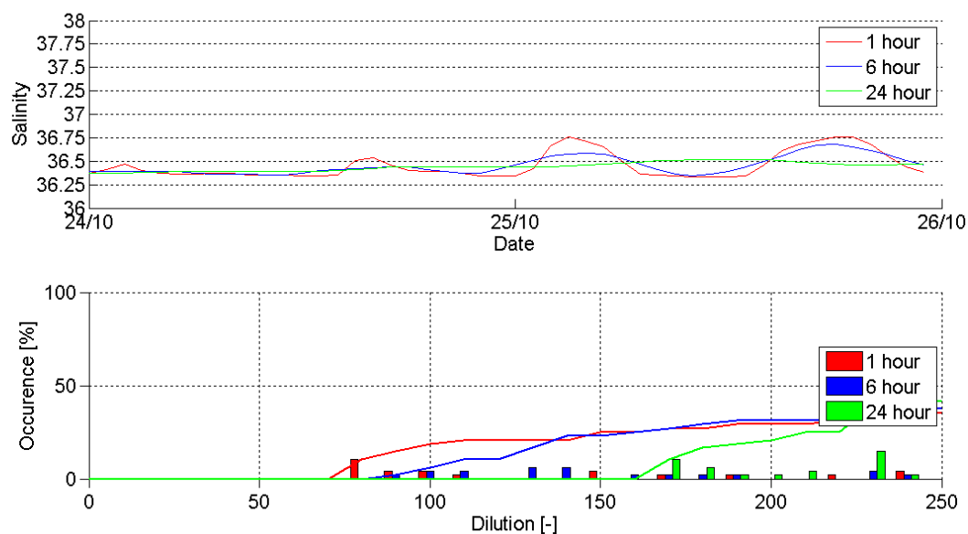
Figure 2 Modelled Inshore Arc 1, Salinity and Dilution Values during the Dodge Tide (24/10/2012 – 26/10/2012)
