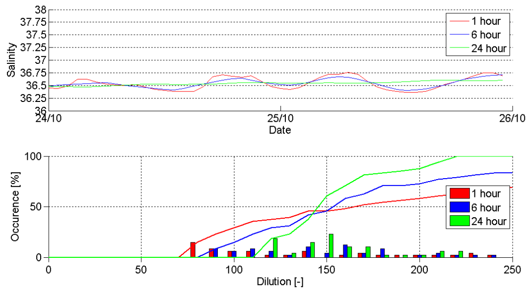
Figure 6 Modelled Offshore Arc 2, Salinity and Dilution Values during the Dodge Tide (24/10/2012 – 26/10/2012)
