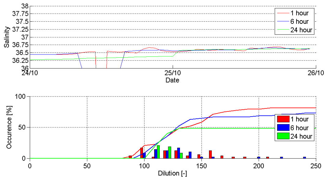
Figure 1 Measured Inshore Arc 1. Salinity and Dilution Values during the Dodge Tide (24/10/2012 – 26/10/2012)
