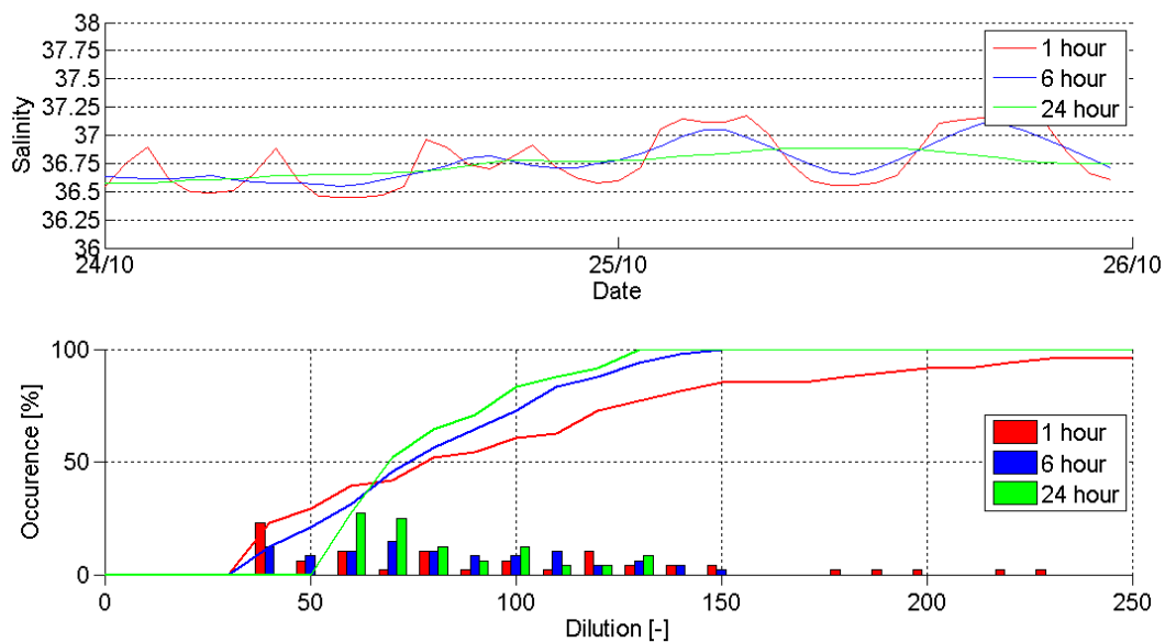
Figure 4 Modelled Offshore Arc 1, Salinity and Dilution Values during the Dodge Tide (24/10/2012 – 26/10/2012)
